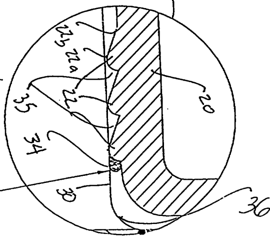
Silicone ring after cap placement
