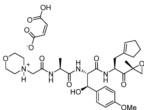
Monomaleate Salt (formed)
