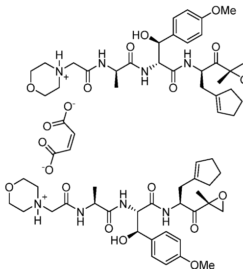
Bridged Maleate Salt (not formed)
