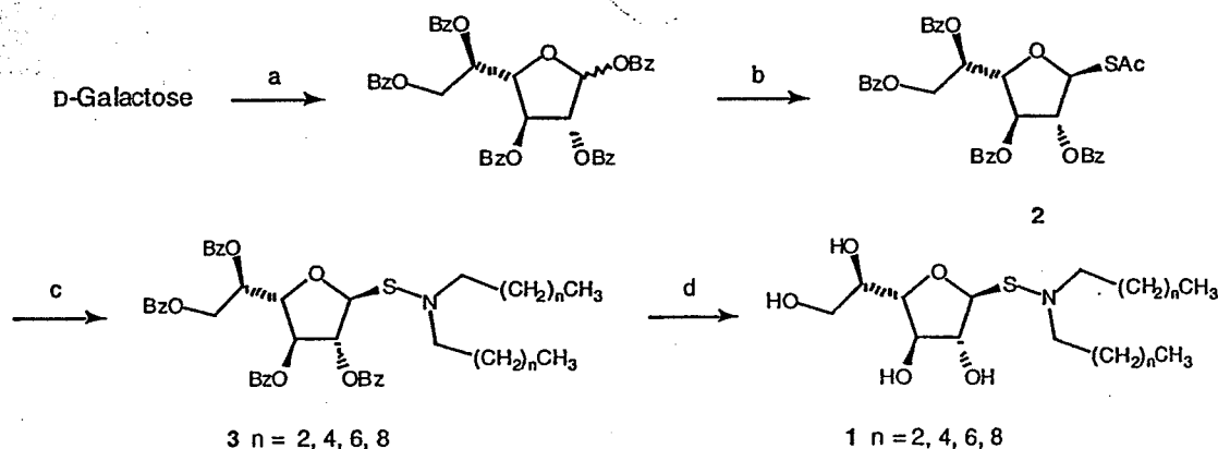
Scheme 1
