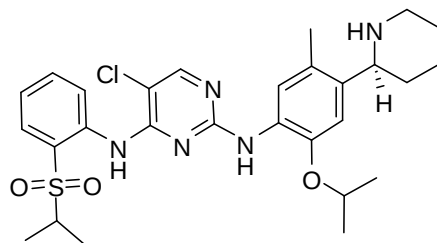
(S)-5-chloro-N2-(2-isopropoxy-5-methyl-4-(piperidin-2-yl)phenyl)-N4-(2-(isopropylsulfonyl)phenyl)pyrimidine-2,4-diamine;
