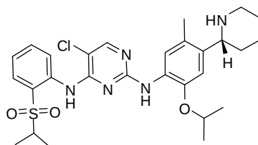
(R)-5-chloro-N2-(2-isopropoxy-5-methyl-4-(piperidin-2-yl)phenyl)-N4-(2-(isopropylsulfonyl)phenyl) pyrimidine-2,4-diamine;
