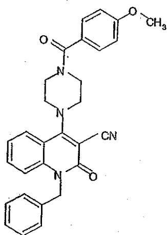
Compound 342
