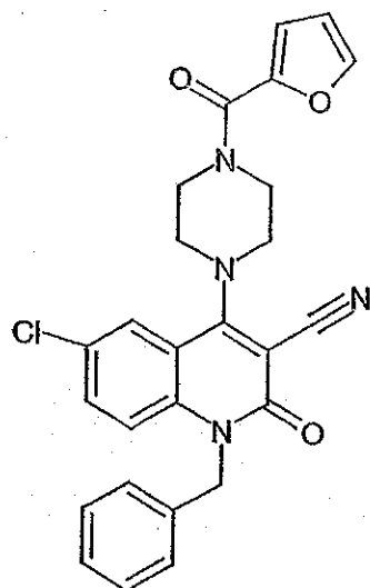
Compound 248
