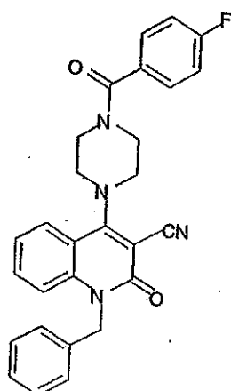
Compound 333
