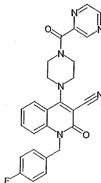
Compound 259
