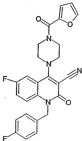
Compound 251
