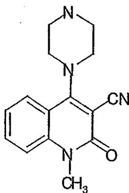
Compound 352
