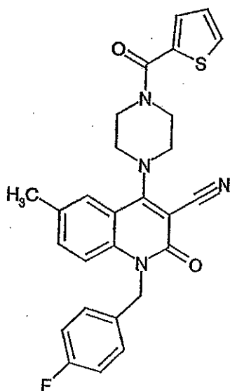
Compound 209
