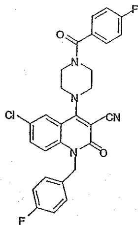
Compound 400
