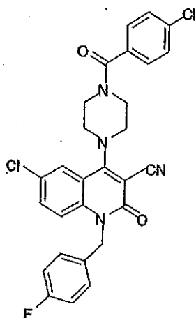
Compound 403
