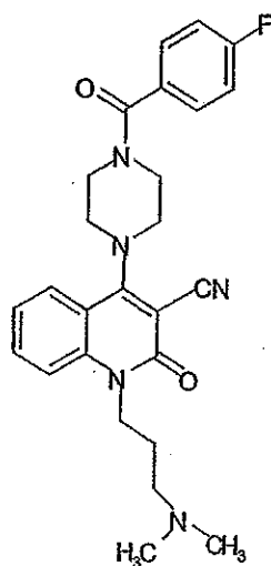
Compound 304
