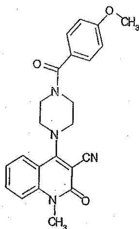
Compound 385
