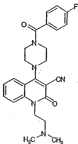
Compound 463
