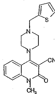
Compound 380
