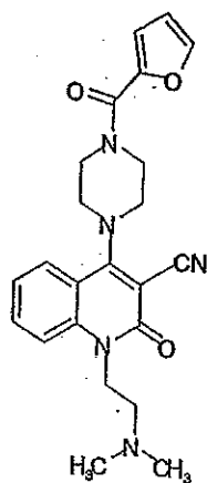
Compound 364
