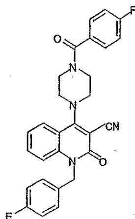
Compound 321
