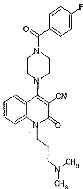
Compound 446
