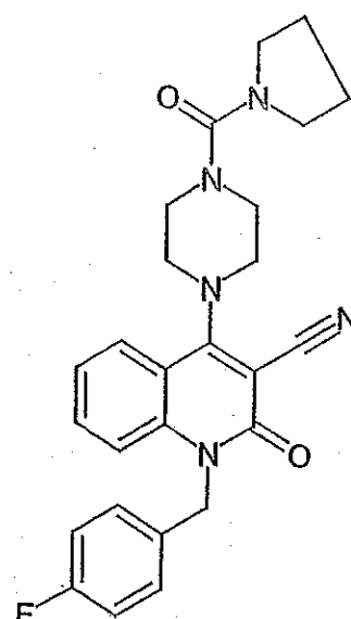
Compound 220
