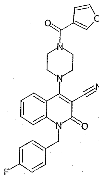
Compound 226
