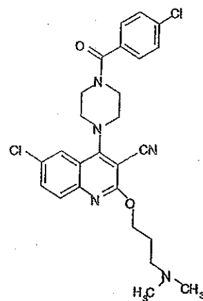
Compound 368
