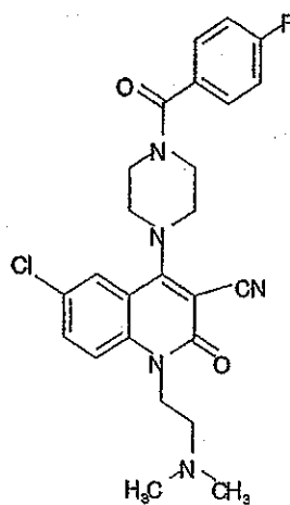
Compound 470
