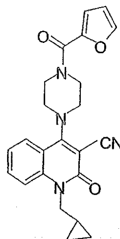
Compound 350
