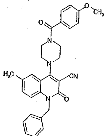
Compound 363
