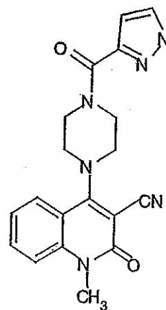
Compound 405
