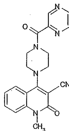
Compound 471
