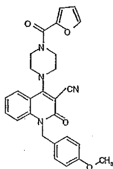
Compound 485
