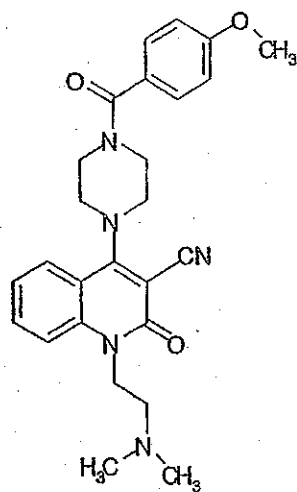
Compound 460
