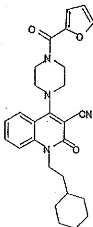
Compound 482
