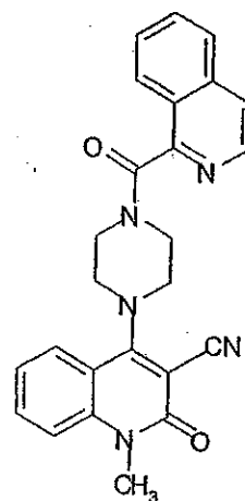
Compound 423
