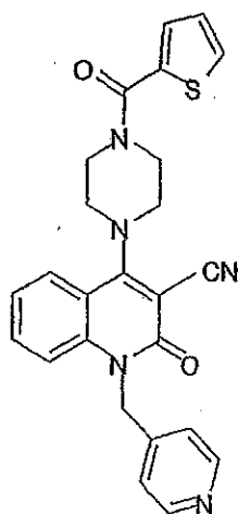
Compound 434
