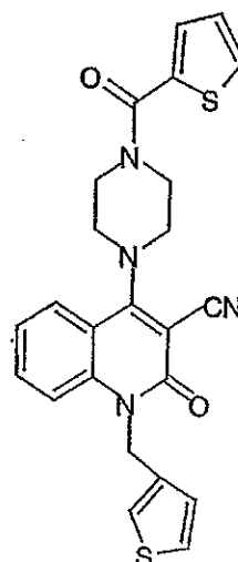
Compound 305
