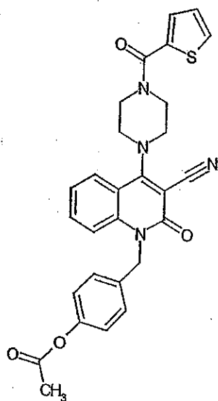
Compound 221
