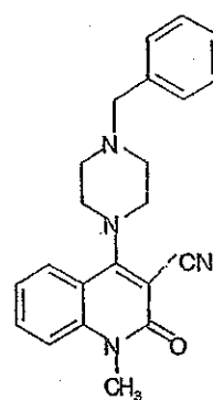
Compound 462
