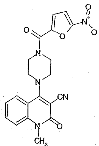
Compound 314
