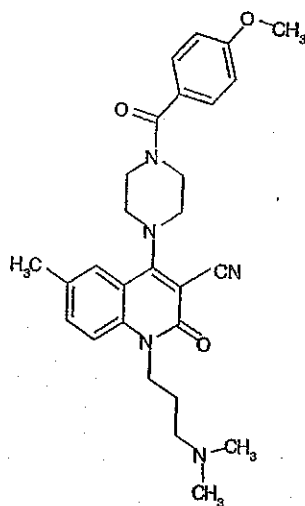
Compound 367
