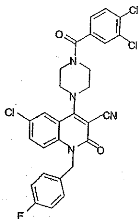
Compound 406
