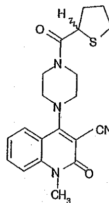
Compound 302
