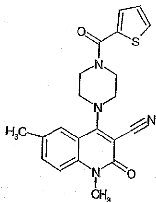
Compound 236
