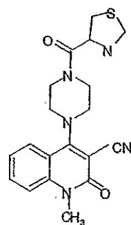
Compound 486
