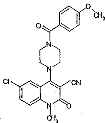
Compound 457
