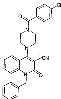
Compound 336
