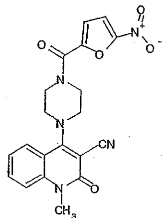
Compound 389
