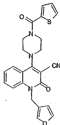
Compound 483
