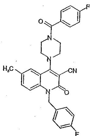
Compound 430
