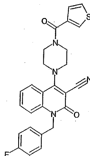
Compound 235
