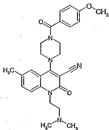
Compound 472
