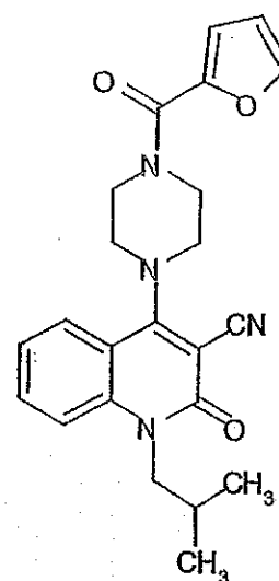
Compound 308
