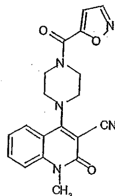
Compound 453
