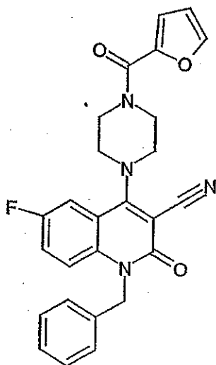
Compound 245
