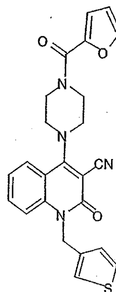
Compound 311
