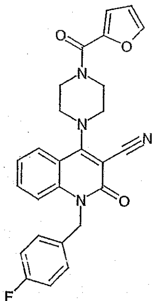
Compound 206
