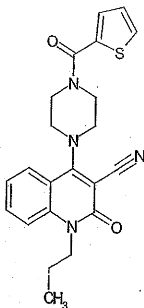
Compound 249
