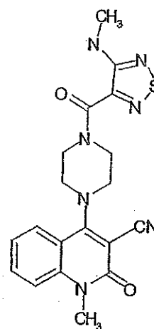
Compound 426
