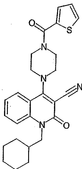
Compound 210
