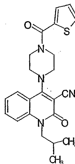
Compound 323
