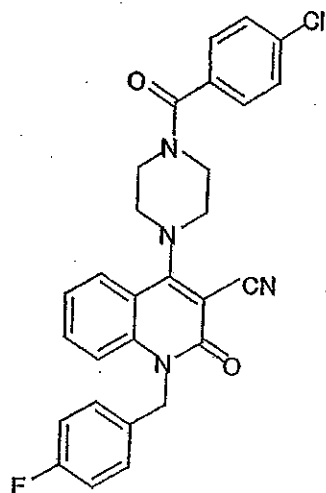
Compound 315
