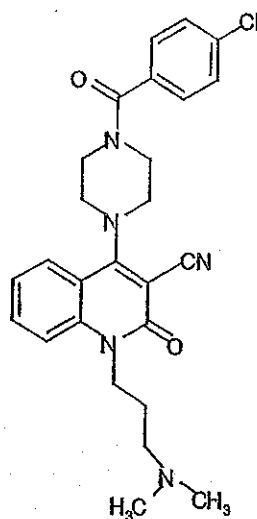
Compound 307
