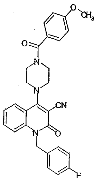
Compound 388
