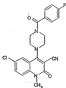
Compound 448
