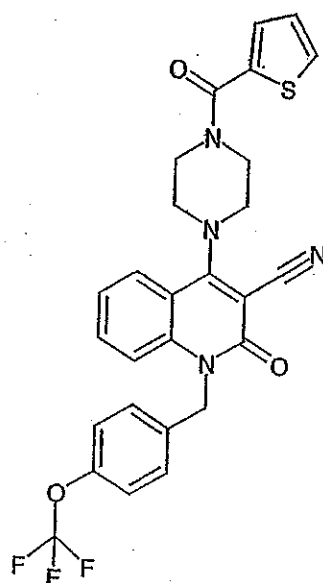
Compound 234
