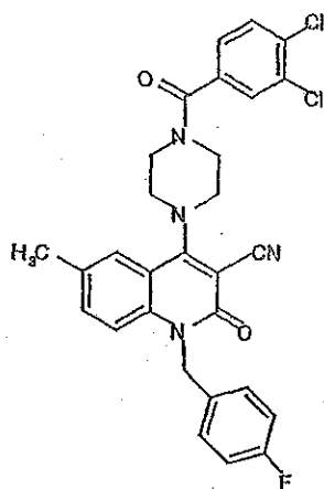
Compound 436
