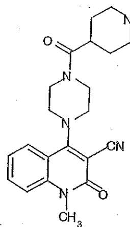
Compound 456
