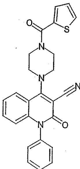
Compound 252
