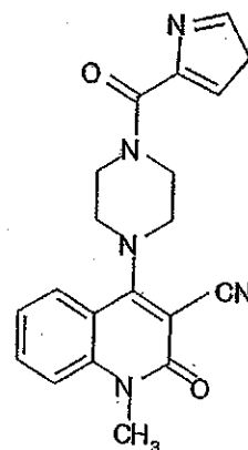
Compound 341
