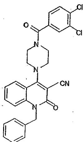
Compound 339
