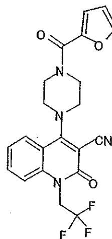
Compound 347
