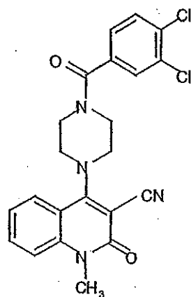
Compound 415
