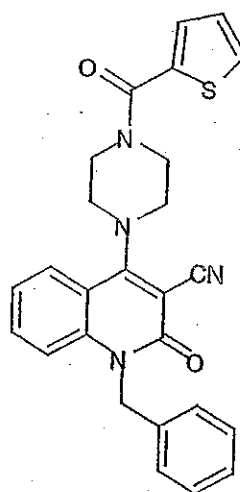
Compound 431
