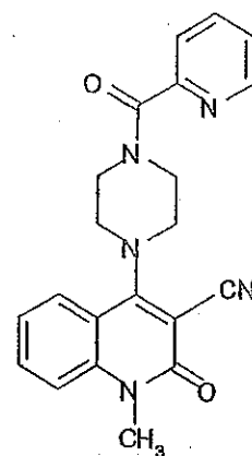
Compound 468
