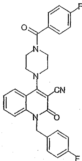
Compound 437
