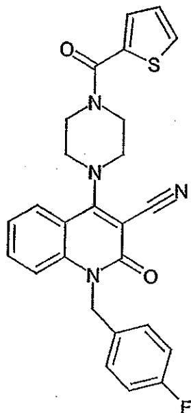
Compound 203
