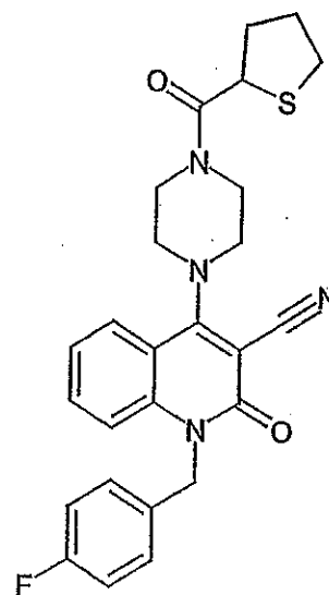
Compound 247
