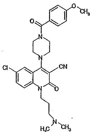
Compound 328
