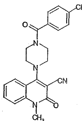
Compound 412
