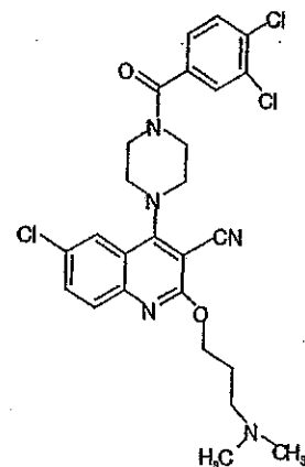
Compound 365
