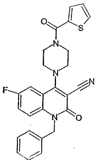
Compound 230
