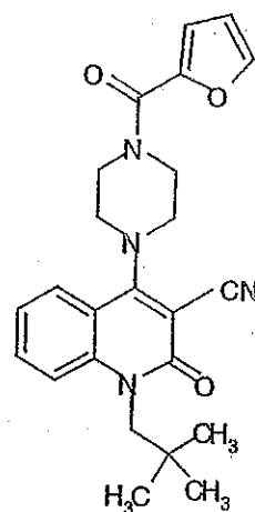
Compound 344
