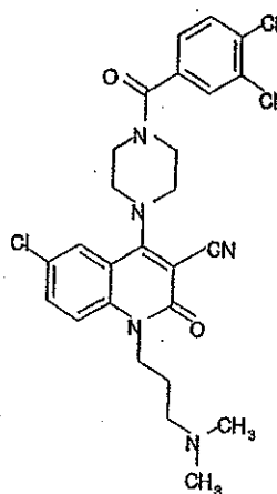
Compound 358
