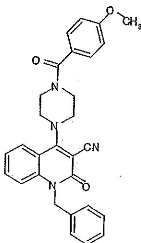
Compound 382
