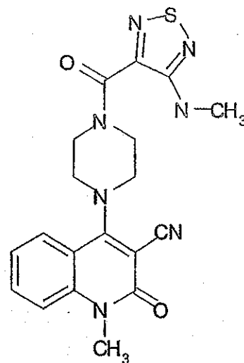
Compound 326
