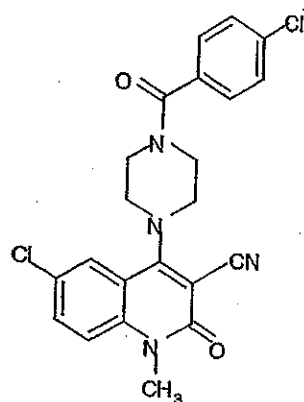
Compound 451
