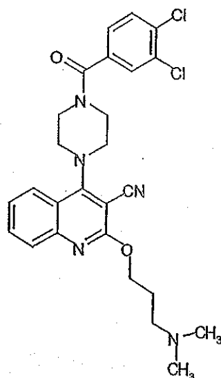
Compound 413
