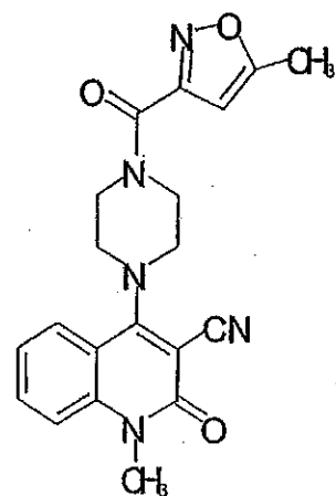
Compound 329
