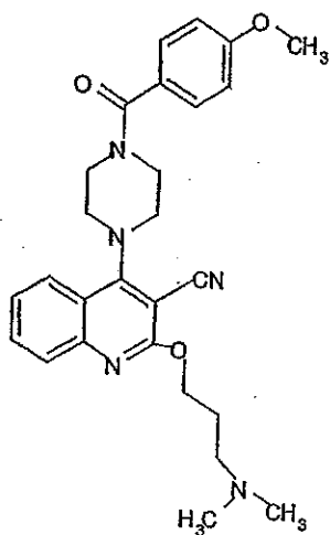
Compound 345
