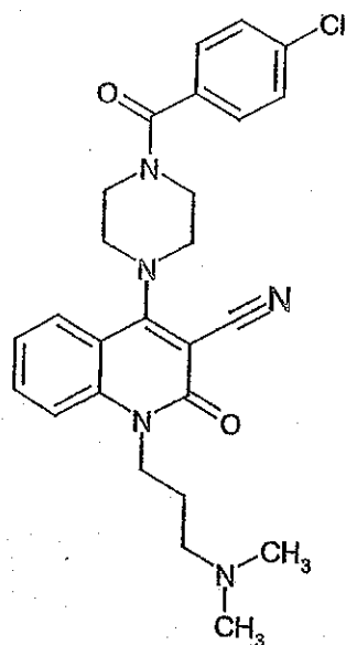
Compound 455
