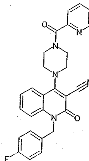
Compound 238
