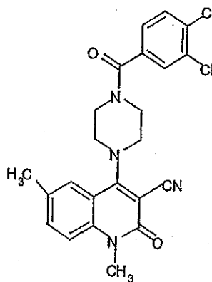
Compound 301
