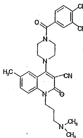
Compound 464
