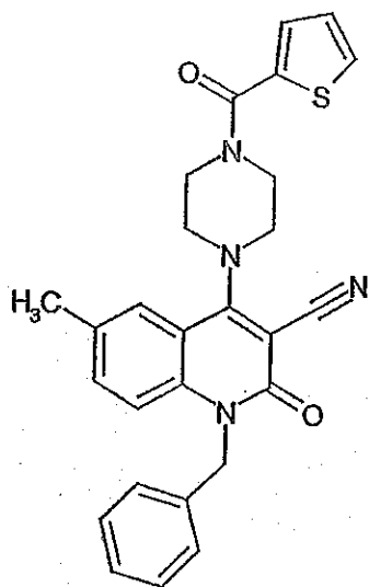
Compound 212
