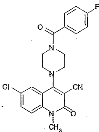
Compound 419
