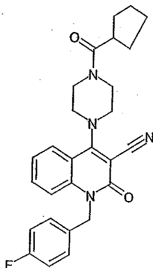
Compound 264
