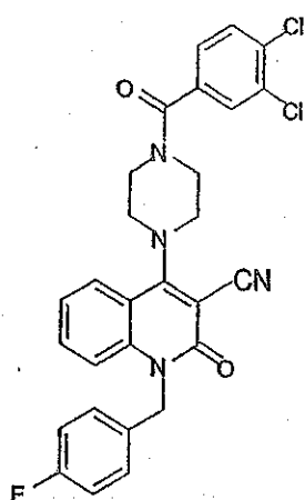
Compound 324
