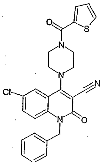
Compound 227
