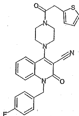
Compound 267
