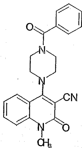
Compound 306
