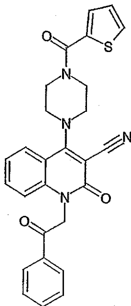
Compound 204
