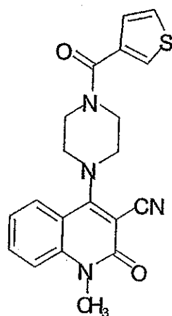
Compound 340
