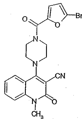
Compound 408
