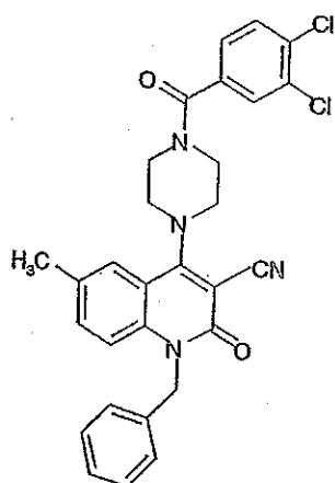
Compound 360
