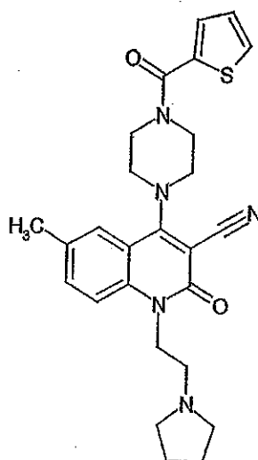
Compound 270
