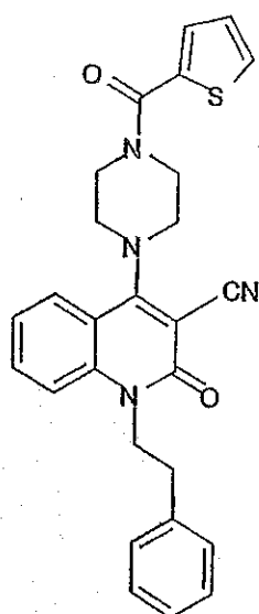
Compound 312
