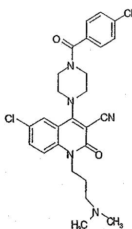
Compound 325
