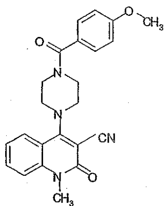
Compound 418
