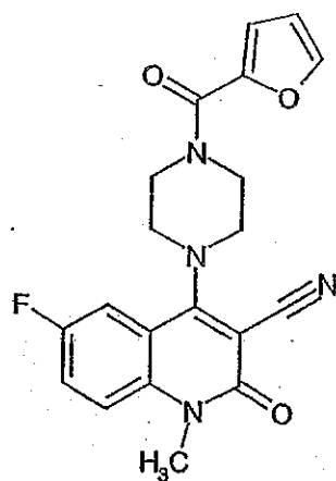
Compound 231
