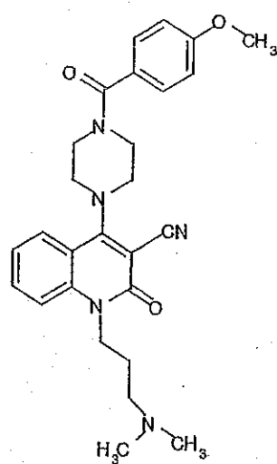
Compound 313
