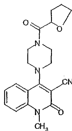
Compound 438
