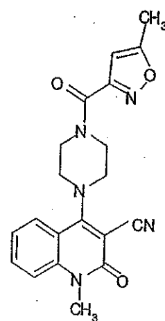
Compound 359
