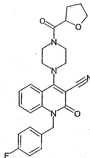
Compound 244
