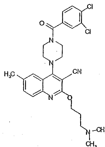
Compound 414
