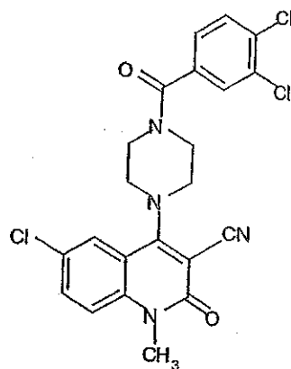
Compound 454
