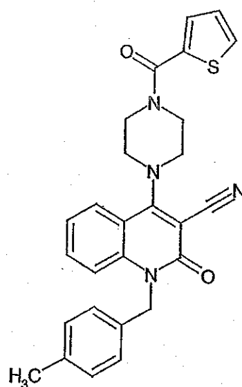
Compound 214
