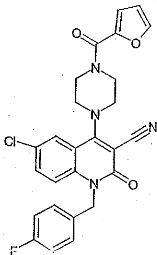
Compound 260
