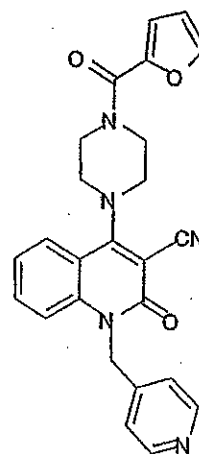
Compound 477
