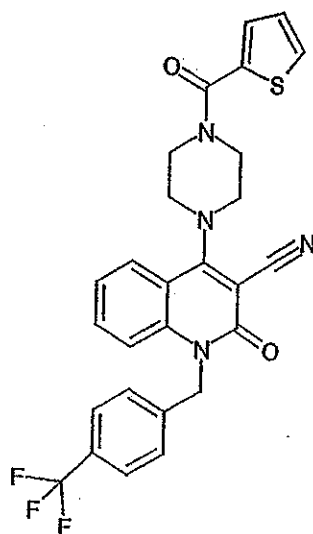
Compound 222
