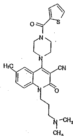
Compound 361
