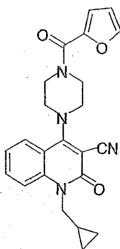
Compound 449
