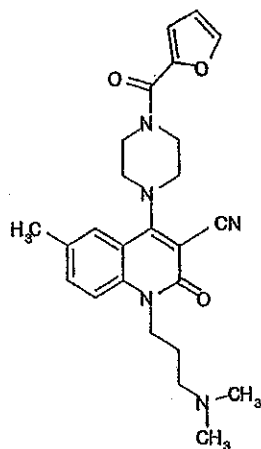
Compound 376
