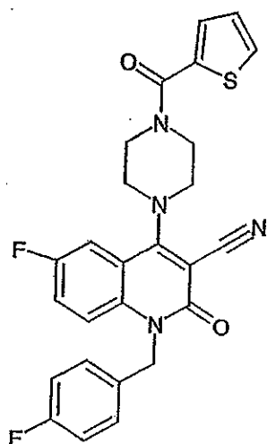
Compound 233
