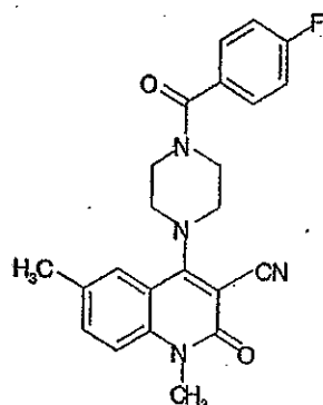
Compound 409
