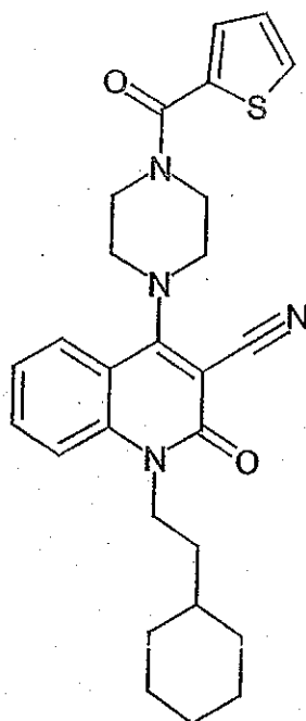
Compound 213
