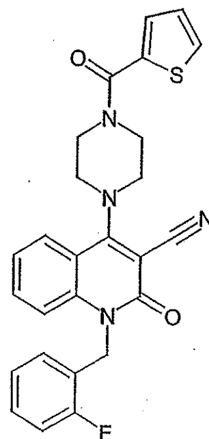
Compound 241
