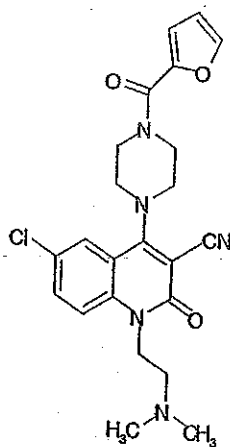
Compound 373
