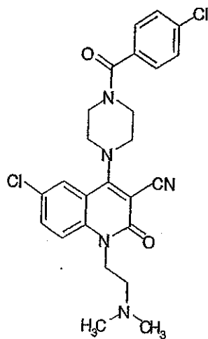
Compound 452
