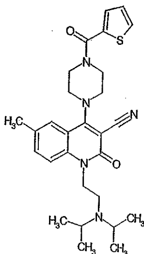
Compound 269
