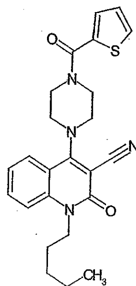
Compound 211
