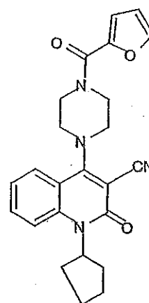
Compound 480
