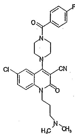
Compound 322
