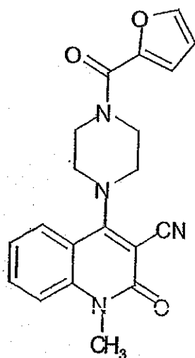
Compound 300
