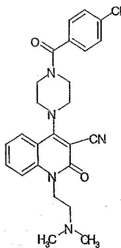
Compound 461
