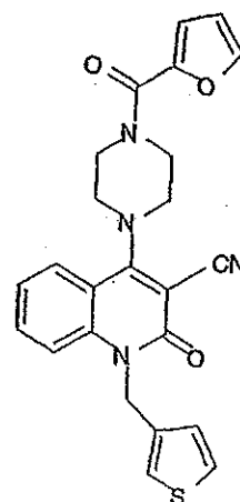
Compound 441
