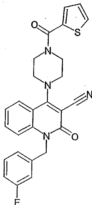
Compound 228
