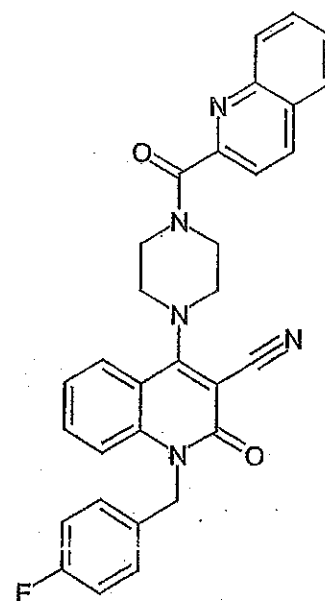
Compound 256
