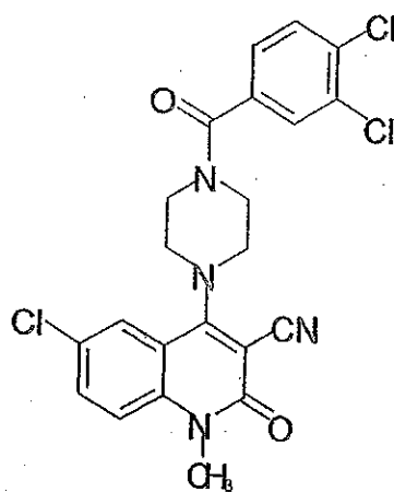
Compound 425
