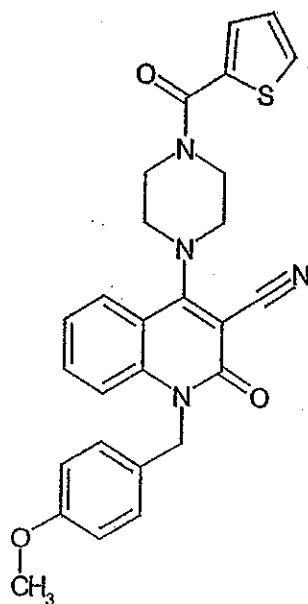
Compound 258
