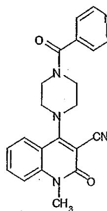
Compound 417
