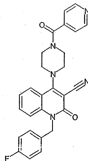
Compound 208
