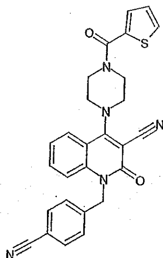
Compound 237
