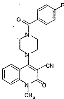
Compound 484
