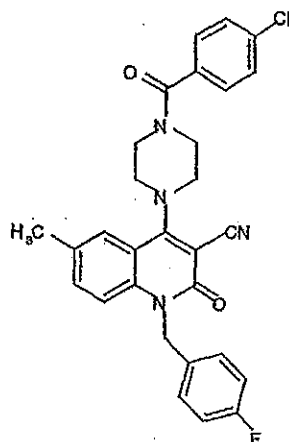
Compound 433
