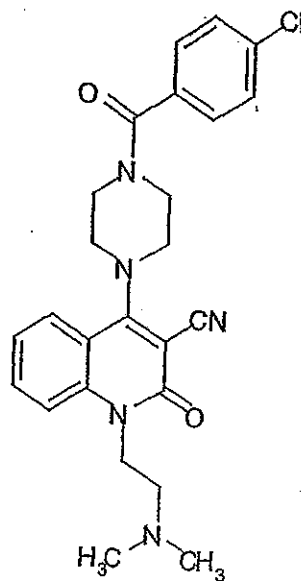
Compound 440
