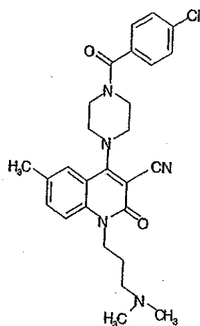
Compound 334
