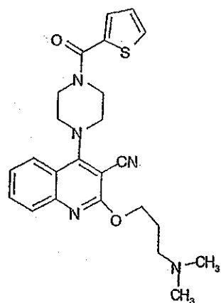
Compound 424
