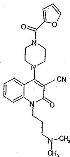
Compound 370
