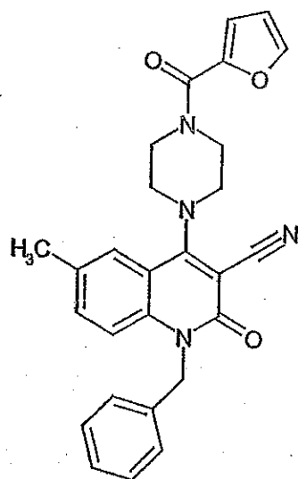
Compound 218
