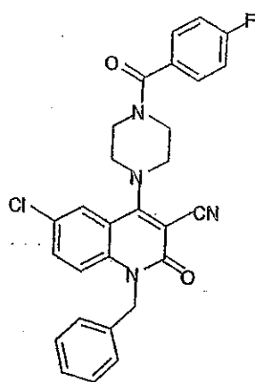
Compound 372
