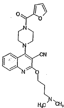
Compound 369
