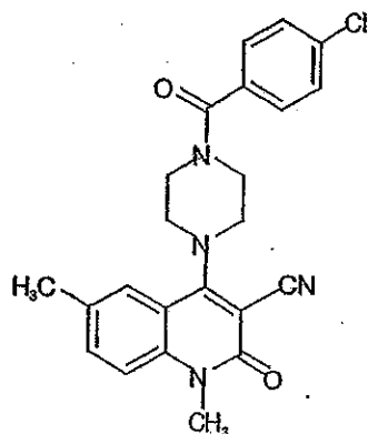
Compound 475
