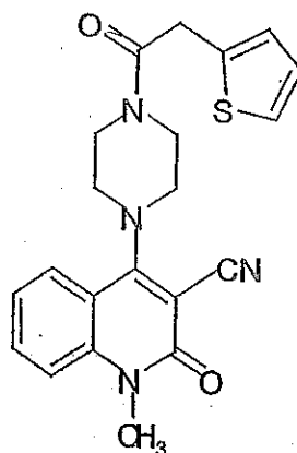
Compound 479
