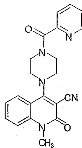
Compound 332
