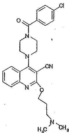
Compound 331
