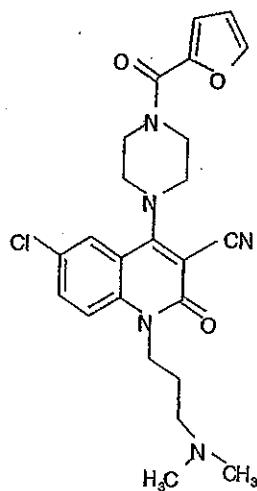
Compound 316
