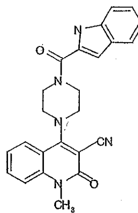
Compound 420
