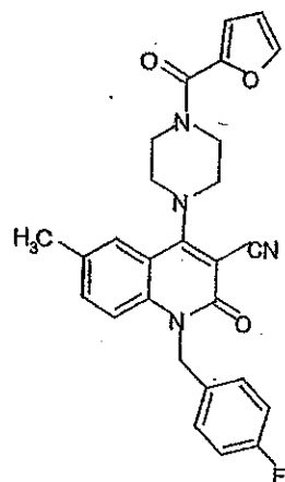
Compound 421
