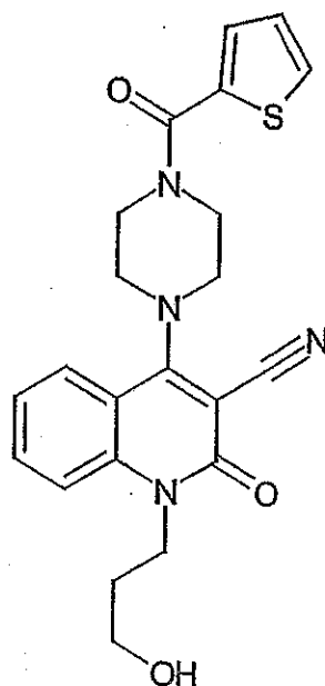
Compound 240
