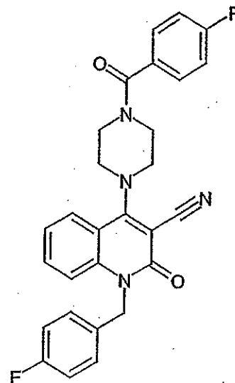
Compound 205
