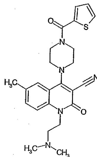
Compound 265
