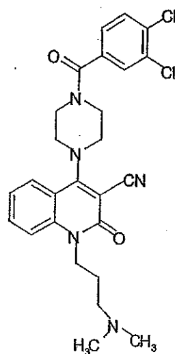
Compound 310
