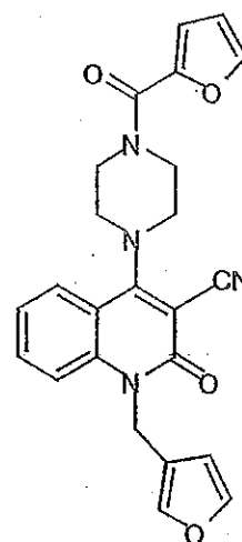
Compound 474
