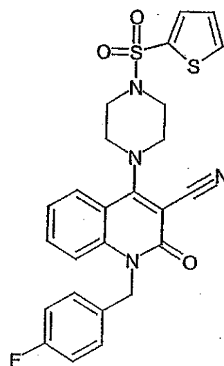
Compound 223
