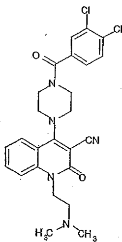
Compound 478
