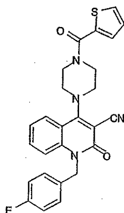
Compound 309
