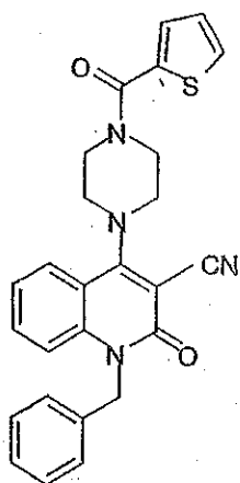
Compound 330
