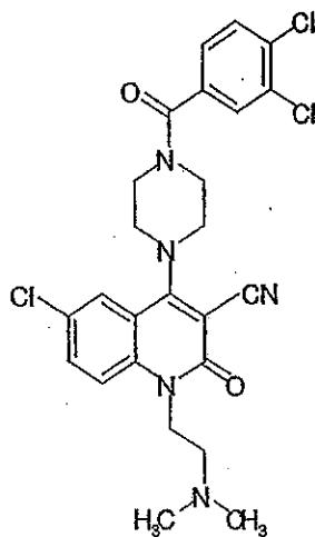
Compound 458
