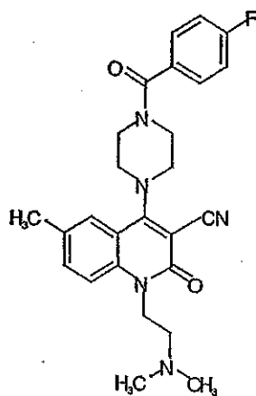
Compound 469
