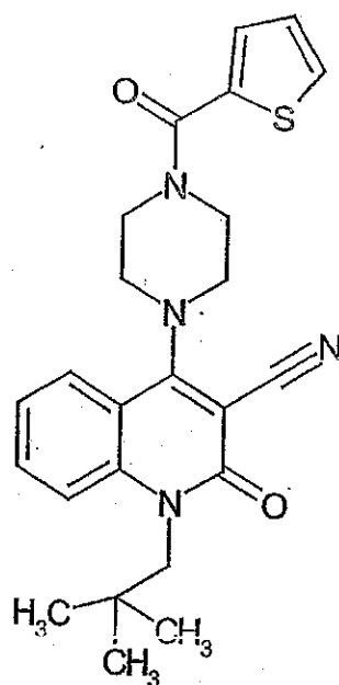
Compound 219
