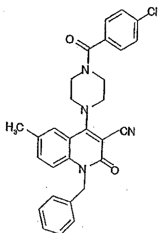
Compound 357
