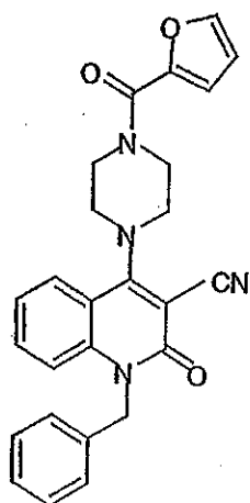
Compound 303
