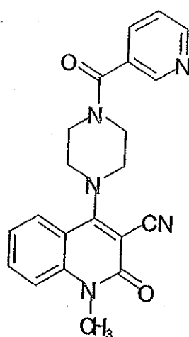
Compound 337
