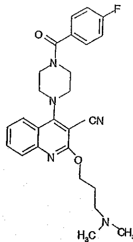
Compound 320
