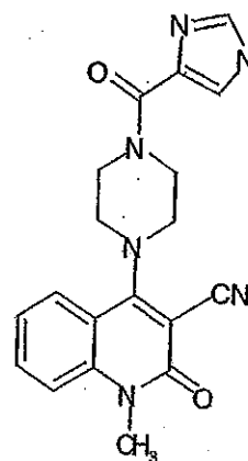
Compound 429
