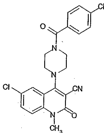
Compound 422
