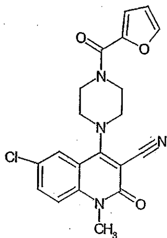
Compound 257
