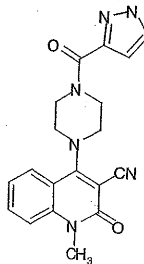
Compound 317
