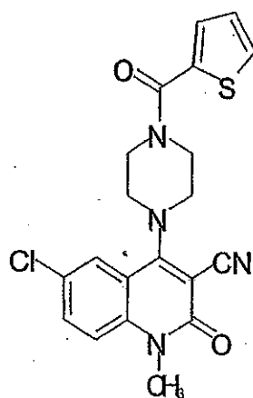
Compound 416
