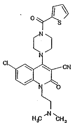
Compound 467
