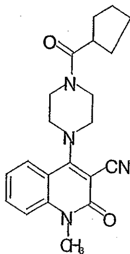
Compound 346
