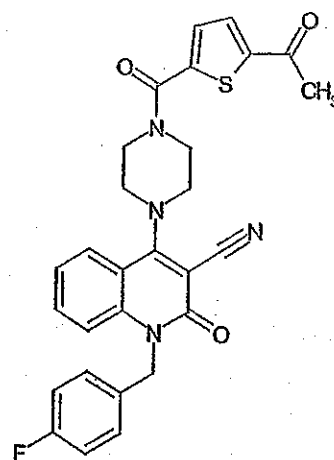
Compound 232
