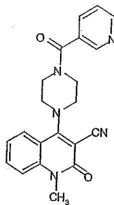
Compound 374
