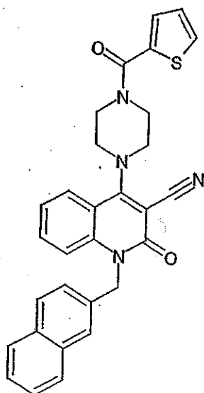
Compound 263
