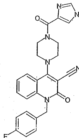
Compound 262
