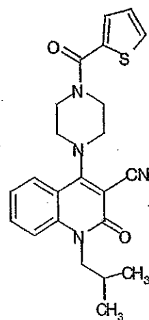
Compound 459
