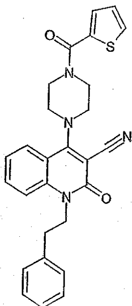
Compound 266
