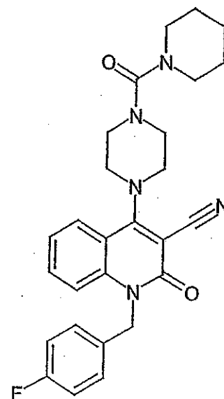
Compound 217
