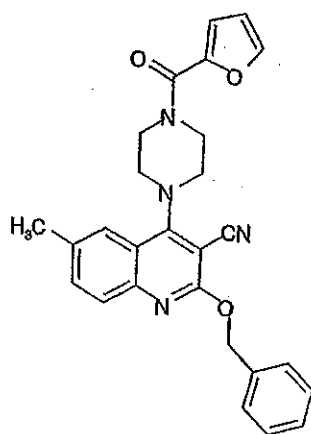
Compound 427
