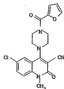
Compound 465
