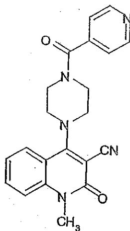
Compound 343
