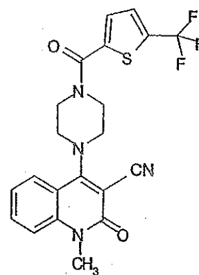
Compound 356
