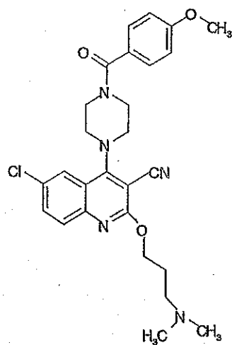
Compound 355
