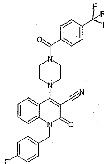
Compound 253
