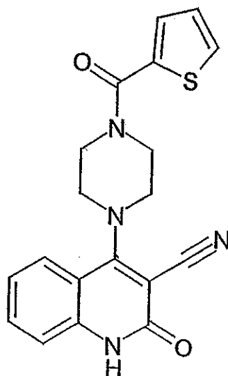
Compound 216
