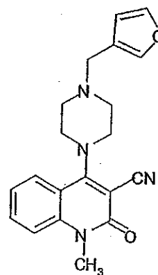
Compound 383
