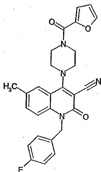
Compound 215
