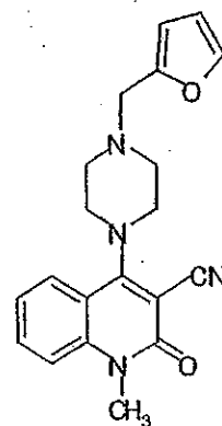
Compound 377
