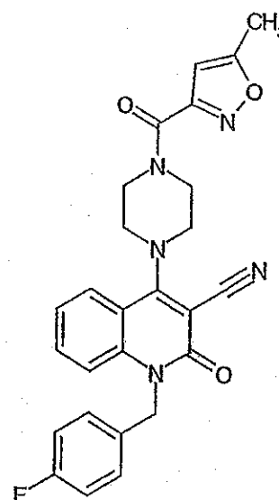
Compound 250
