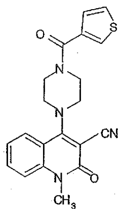
Compound 402
