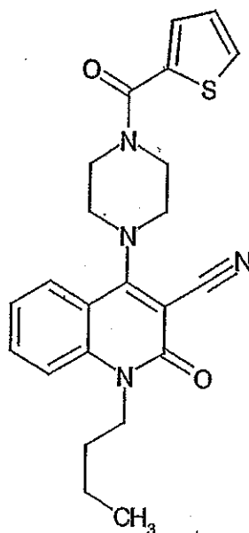
Compound 246
