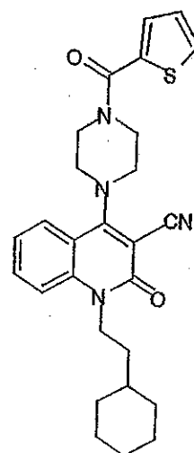
Compound 371
