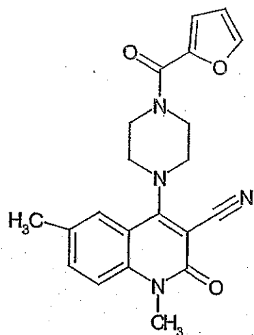
Compound 254
