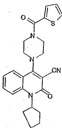
Compound 318
