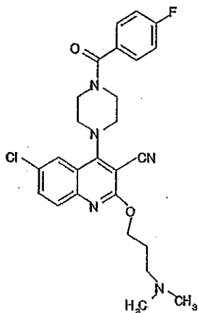
Compound 351
