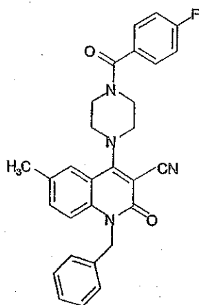
Compound 354
