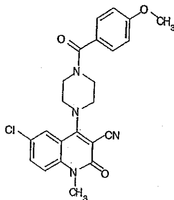
Compound 428
