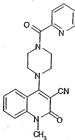
Compound 349
