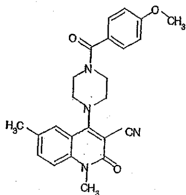
Compound 439
