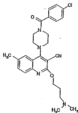
Compound 366
