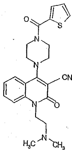
Compound 443
