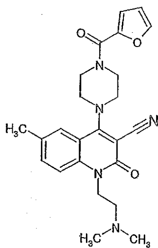
Compound 466
