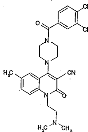
Compound 476
