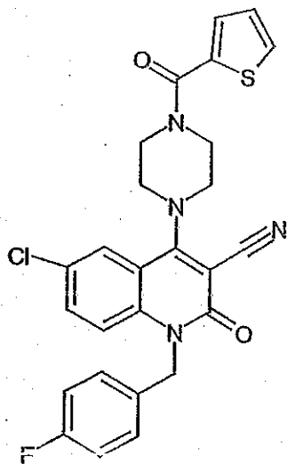
Compound 242
