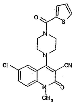
Compound 445
