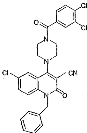
Compound 378
