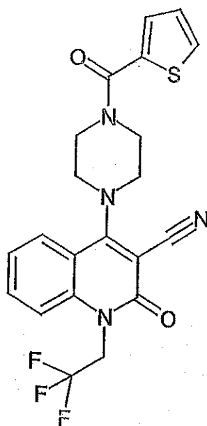
Compound 225
