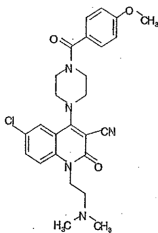
Compound 473
