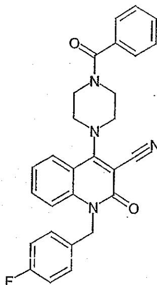
Compound 261
