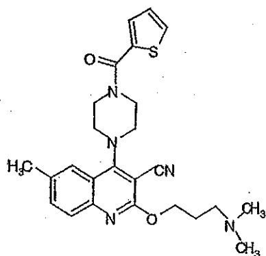
Compound 387
