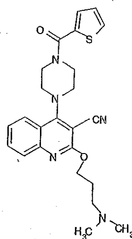
Compound 362
