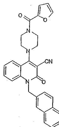
Compound 386
