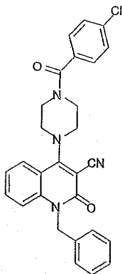
Compound 401
