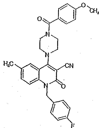
Compound 442
