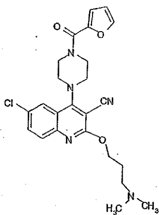
Compound 348
