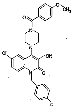
Compound 481
