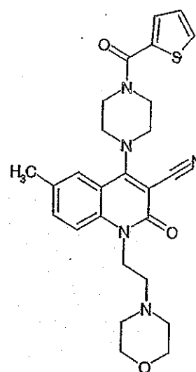
Compound 268
