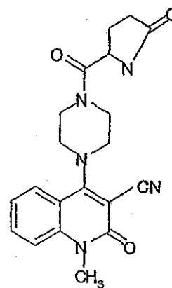
Compound 435
