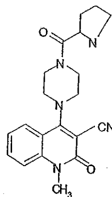
Compound 432
