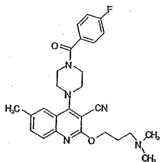
Compound 384
