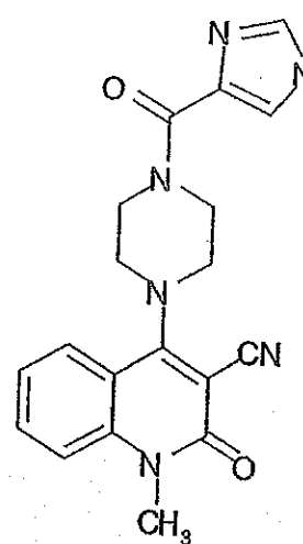
Compound 338
