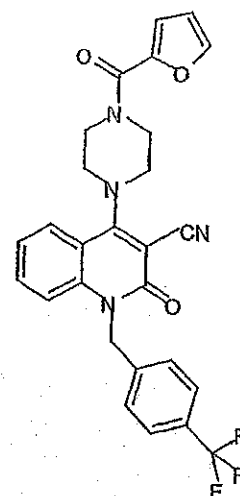
Compound 444
