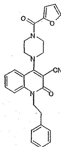
Compound 450
