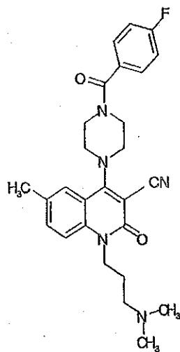
Compound 379
