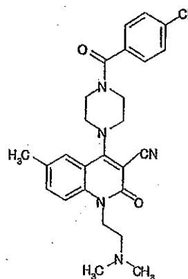
Compound 410
