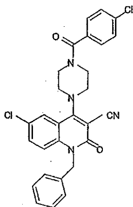
Compound 375
