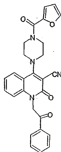
Compound 447
