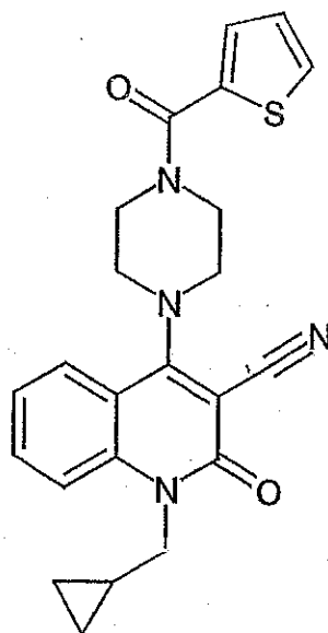
Compound 243
