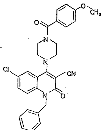
Compound 381
