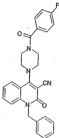
Compound 404
