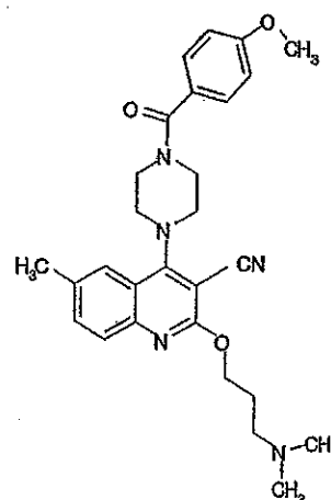
Compound 411
