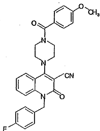
Compound 327
