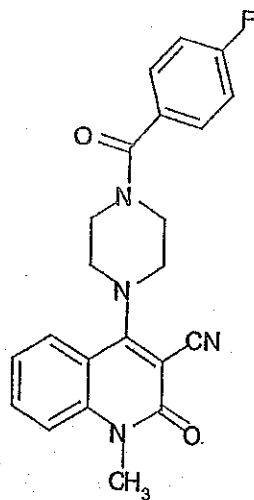
Compound 407
