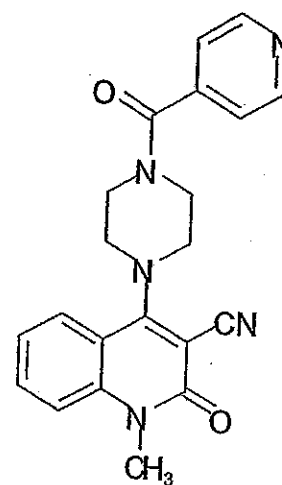
Compound 335
