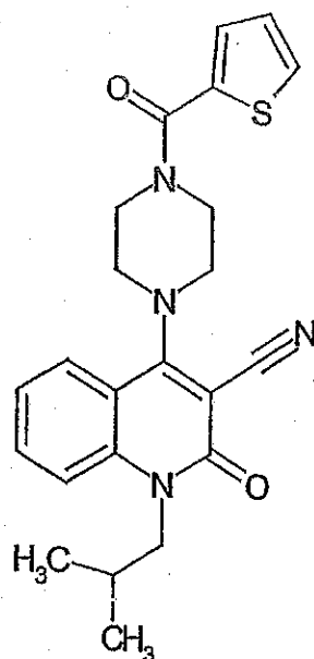
Compound 255
