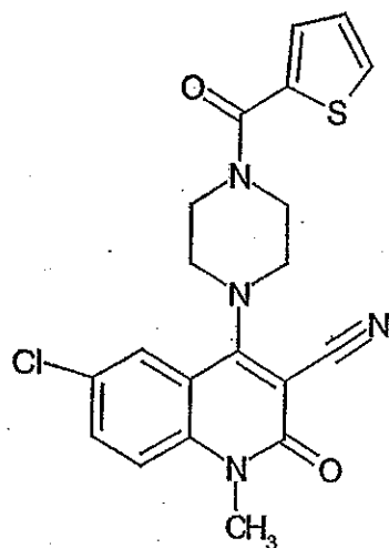
Compound 239
