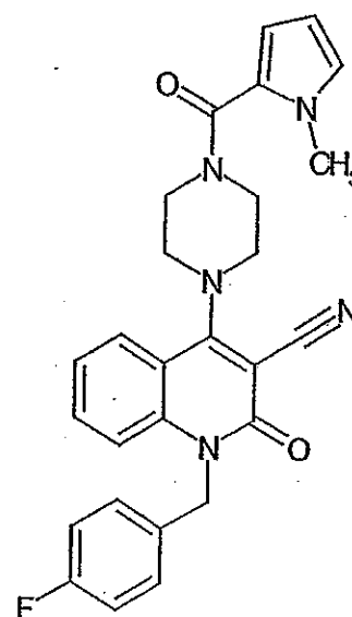
Compound 229
