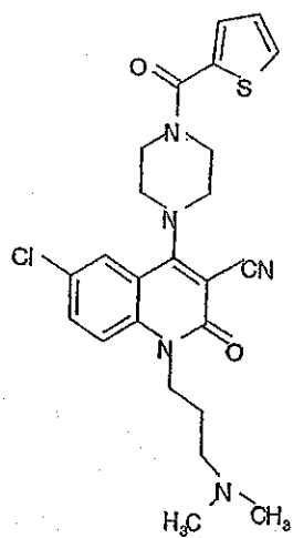
Compound 319
