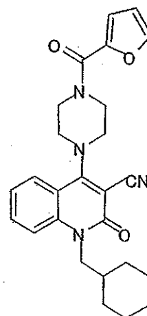
Compound 353
