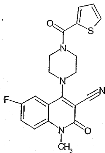
Compound 224
