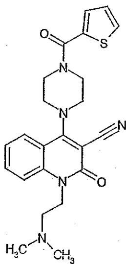
Compound 207
