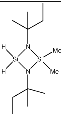
1,3-bis(tert-amyl)-2-dimethylcyclodisilazane
