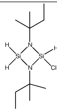
1,3-bis(tert-amyl)-2-chloro-cyclodisilazane
