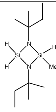
1,3-bis(tert-amyl)-2-methyl-cyclodisilazane
