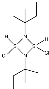
1,3-bis(tert-amyl)-2,4-dichloro-cyclodisilazane
