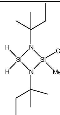
1,3-bis(tert-amyl)-2-chloro-2-methylcyclodisilazane
