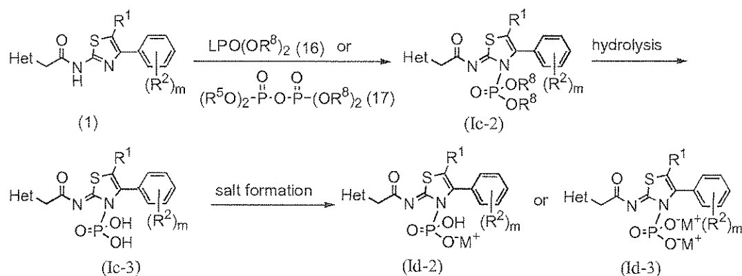
15 Synthetic scheme 9
