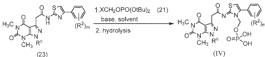
Synthetic scheme 14
