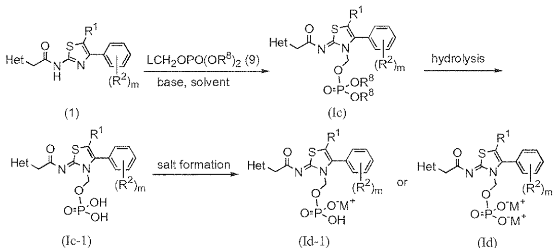
Synthetic scheme 5
