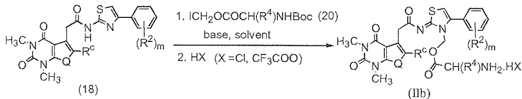
Synthetic scheme 11
