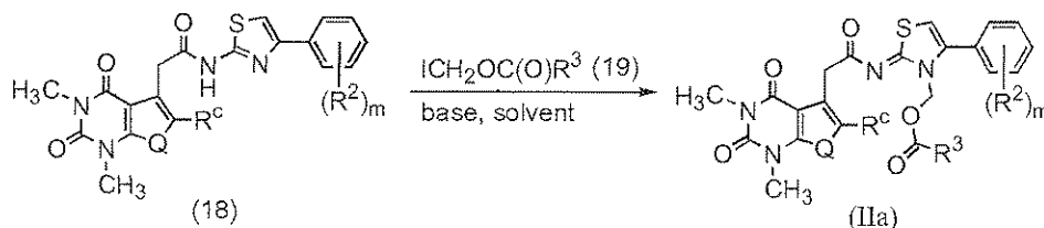
Synthetic scheme 10
