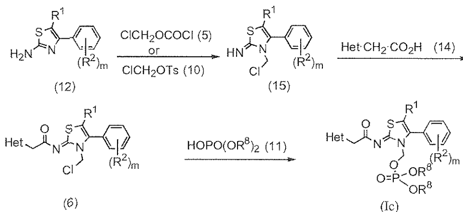
Synthetic scheme 8
