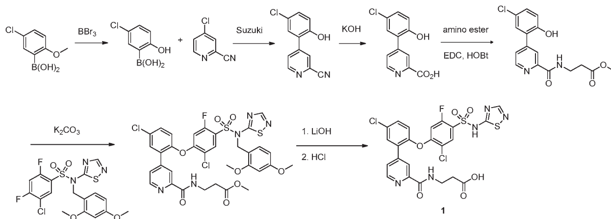
Scheme 5
