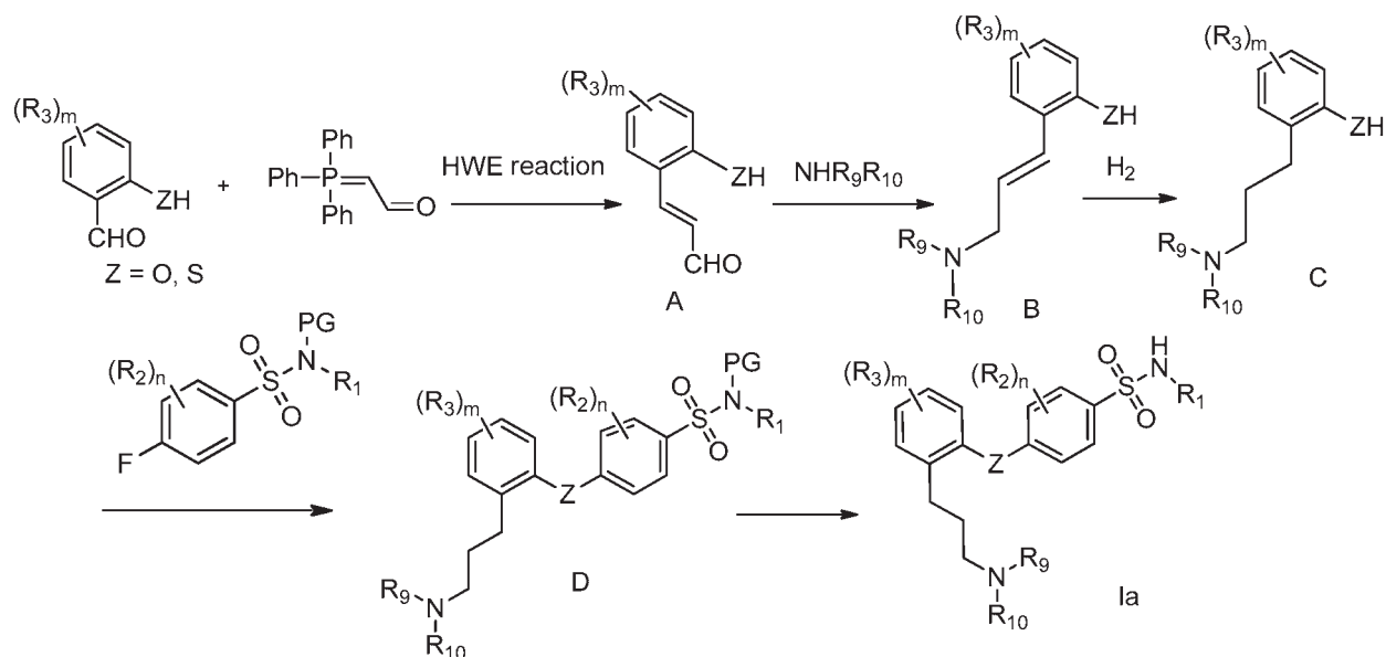
Scheme 1
