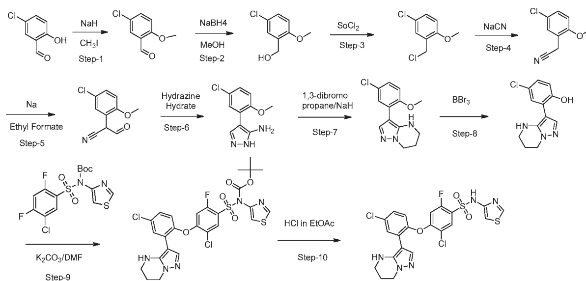
Scheme 13
