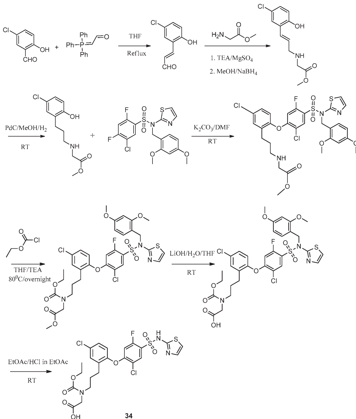
Scheme 14
