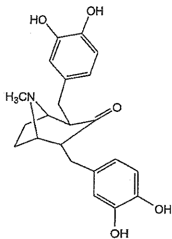
2,4-bis(3,4-dihydroxybenzyl)-8-methyl -8-aza-bicyclo[3.2.1]octan-3-one
