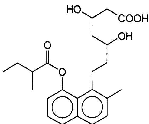
Lovastatin - hydroxy acid
