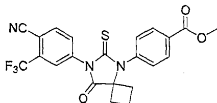
Formula 25
