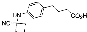
Formula 50
