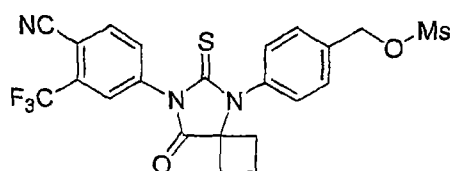
Formula 22
