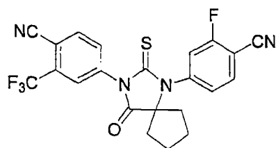
Formula 30
