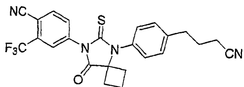
[RD170]
