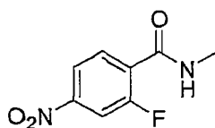
Formula 38
