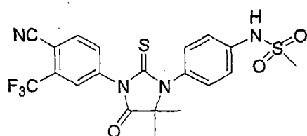
Formula 2
