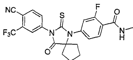
[RD162'']
