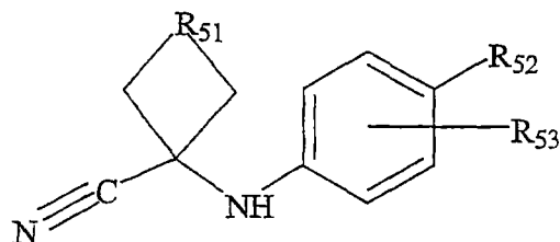
Compound II
