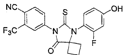
Formula 29
