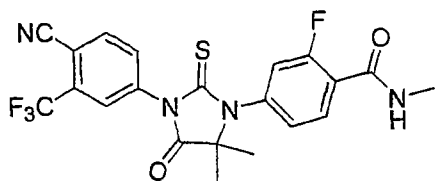
RD162' (Formula 42)
