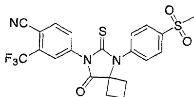
Formula 14
