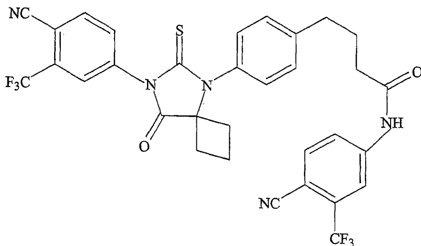
5 Formula 36 [RD142]
