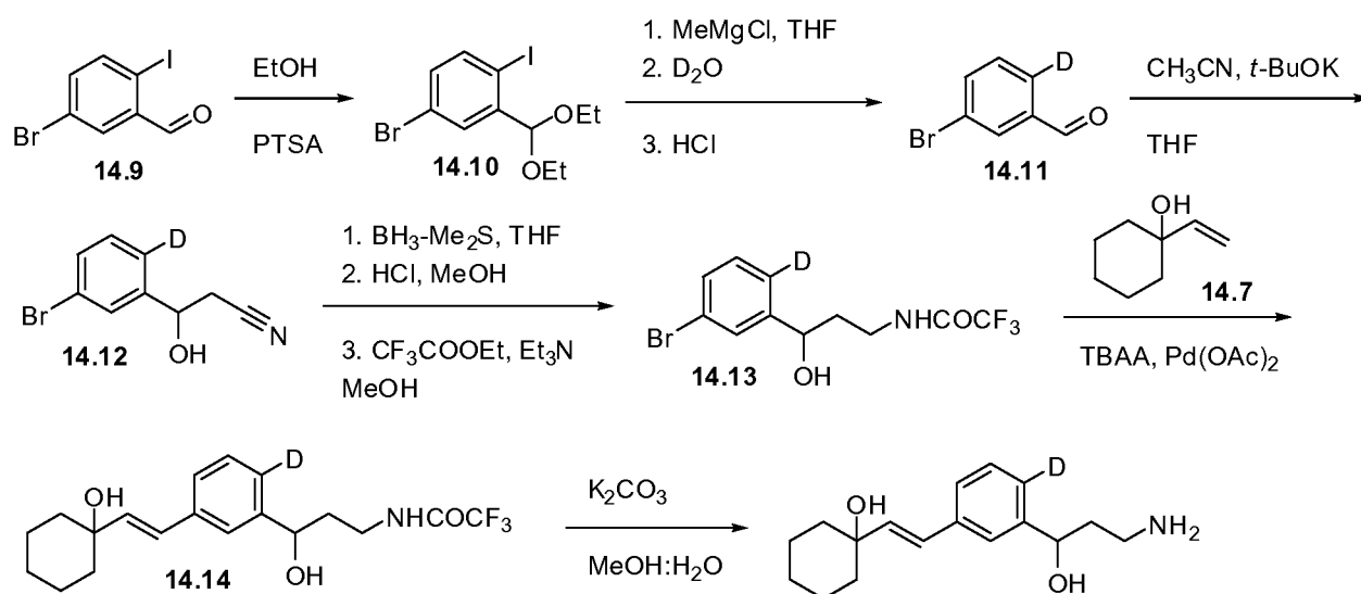
SCHEME 14
