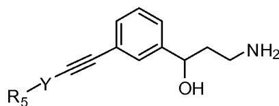
Formula (IIIa)
