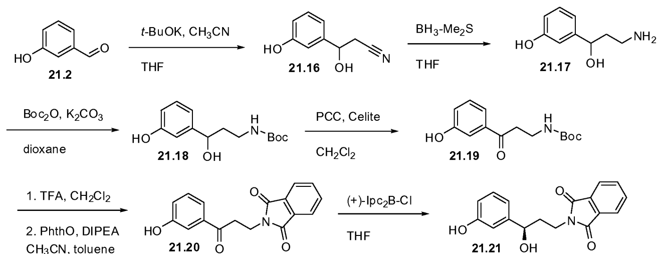
SCHEME 21a
