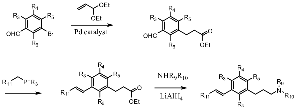
SCHEME II
