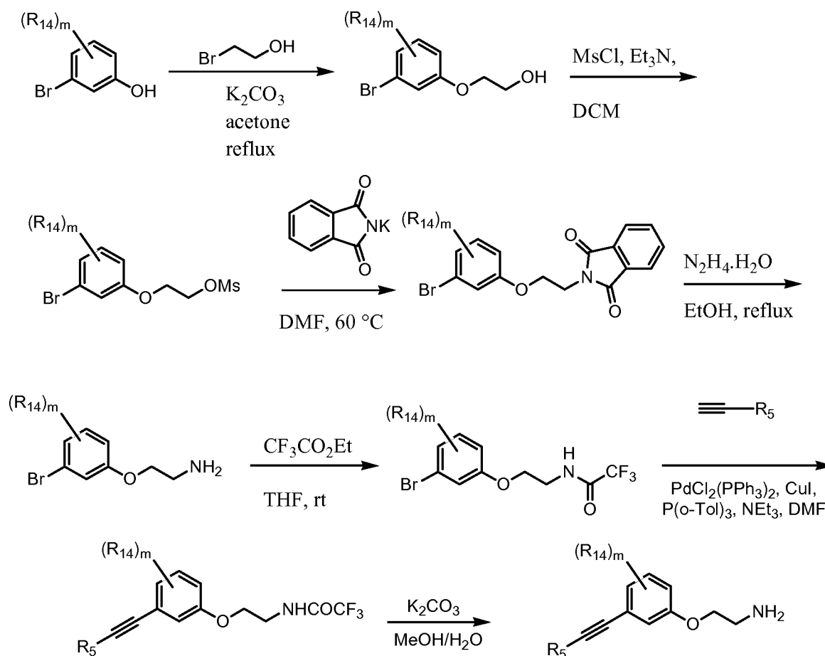
Scheme II
