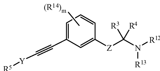
Formula (III)
