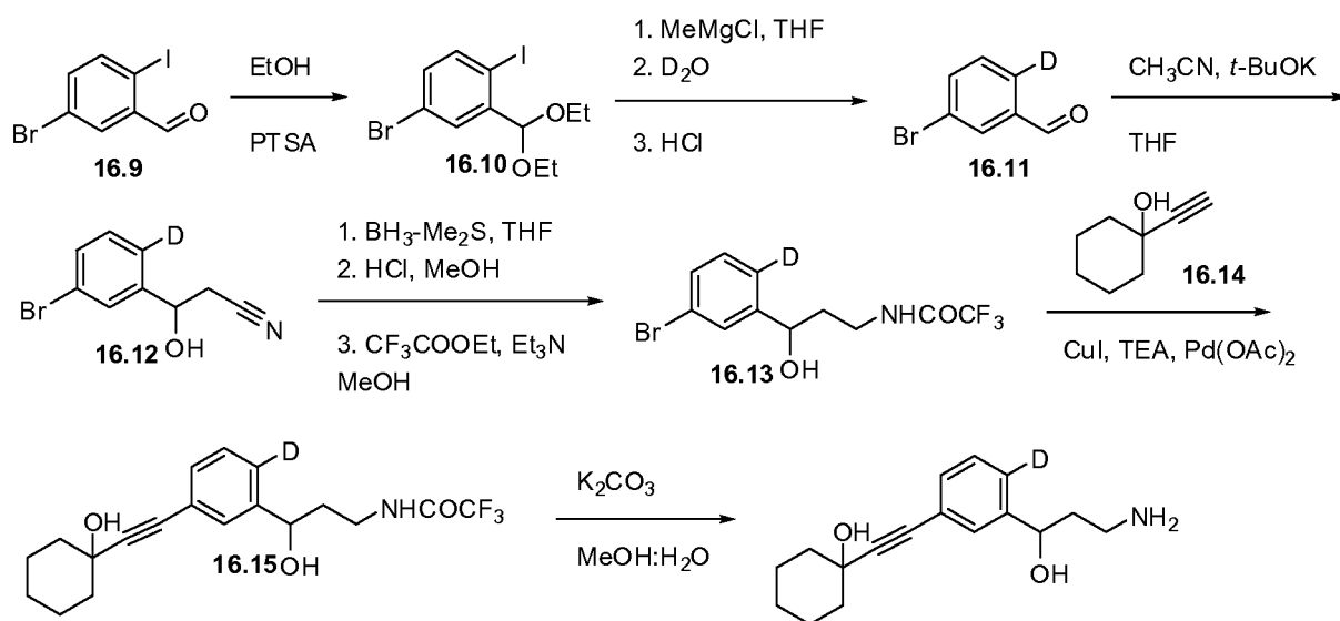
SCHEME 16
