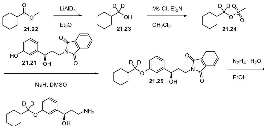
SCHEME 21b
