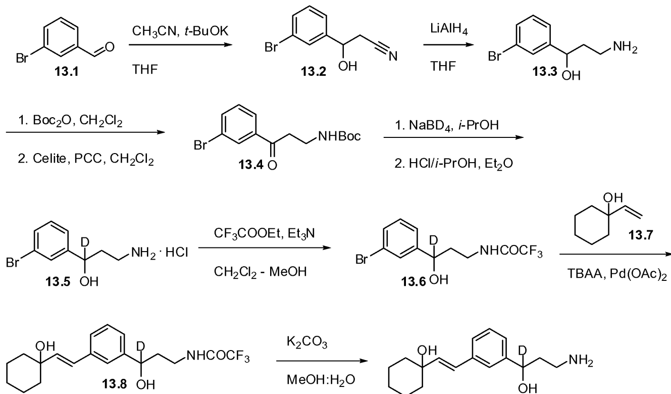
SCHEME 13
