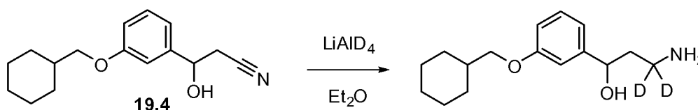
SCHEME 19
