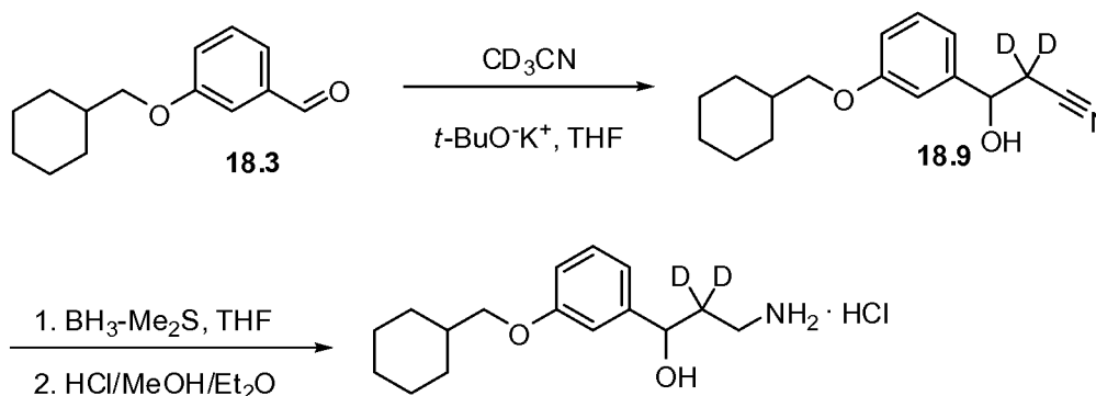
SCHEME 18
