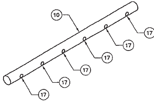
FIGURE 4a. DETAIL DIRECT RECYCLE PIPE (HOLES)
