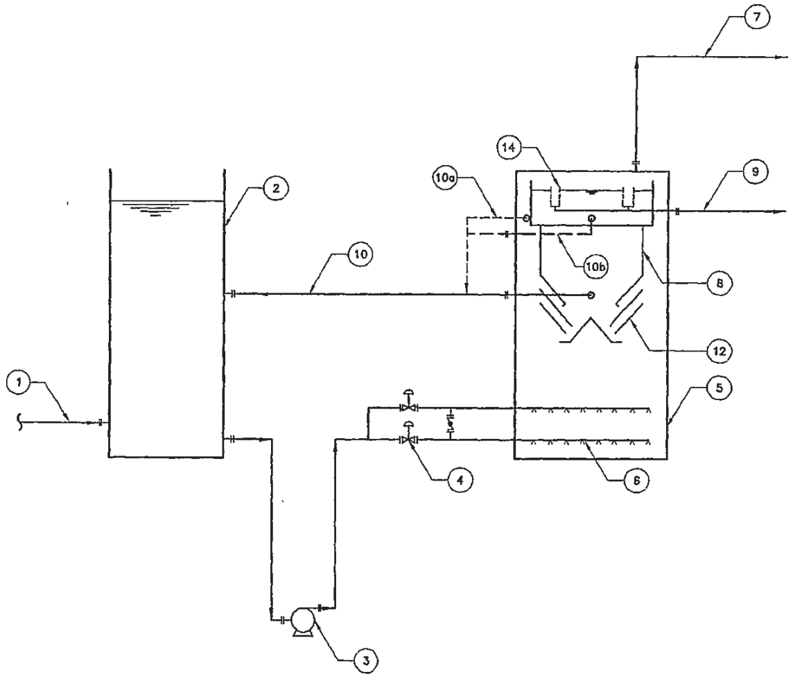
FIGURE 1. GENERAL PROCESS ARRANGEMENT
