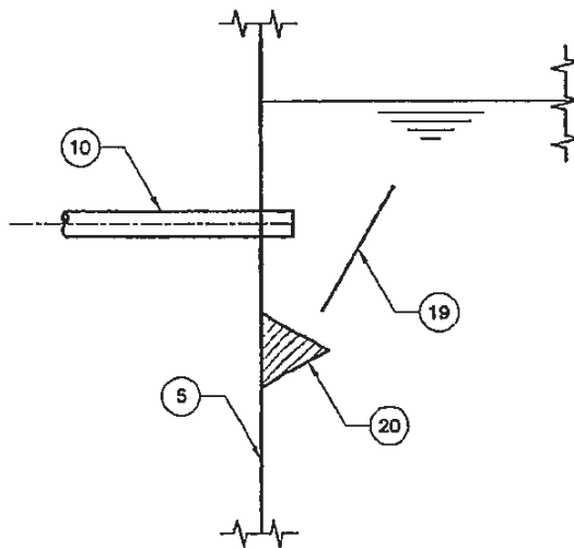
FIGURE 6. GAS DEFLECTING DEVICE
