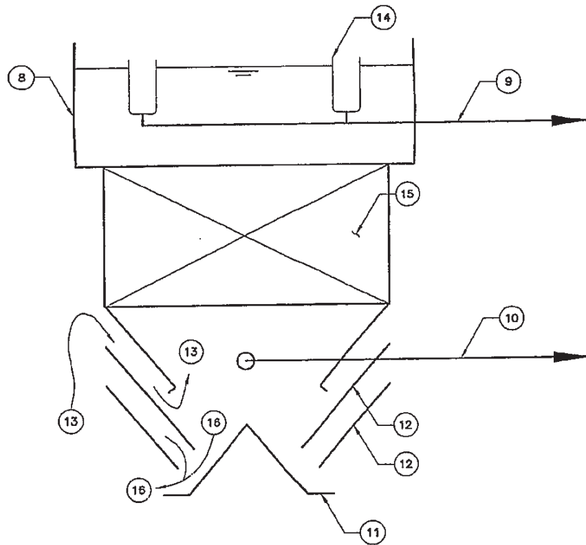
FIGURE 2a. THREE PHASE SEPARATOR
