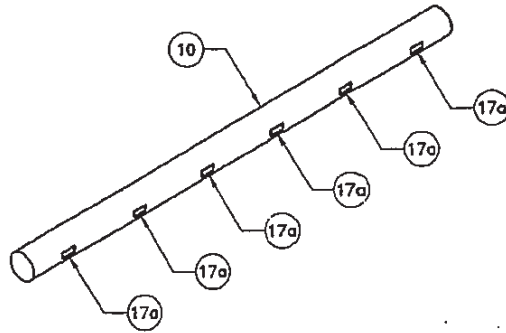
FIGURE 4b. DETAIL DIRECT RECYCLE PIPE (SLOTS)
