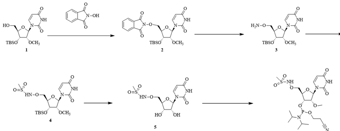
Example 6 Monomer
