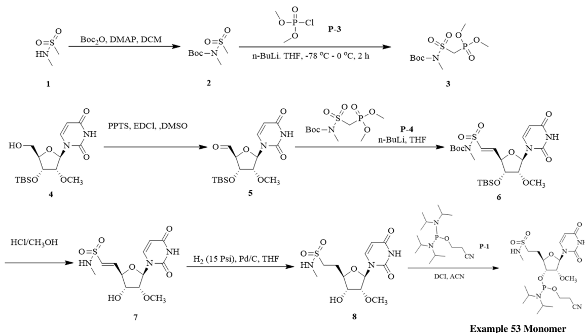
Example 53 Monomer
