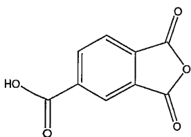
(trimellitic anhydride—TMA)
