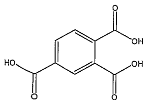
(trimellitic acid—TMLA)
