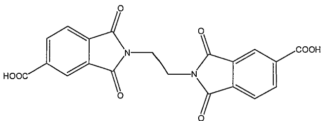
(TMA-EDA imide)
