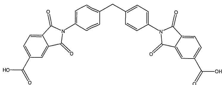
(TMA-MDA imide)
