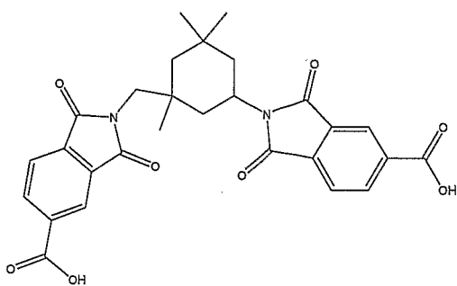
(TMA-IPDA imide)
