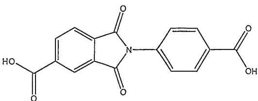
(TMA-PABA imide)
