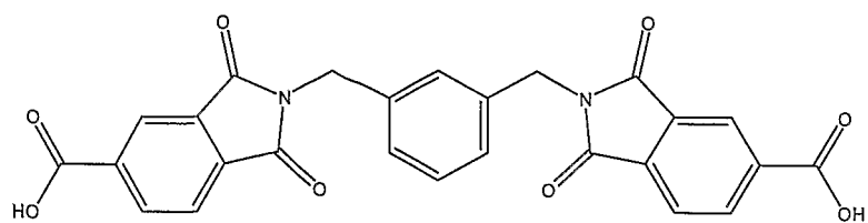
(TMA-MXDA imide)
