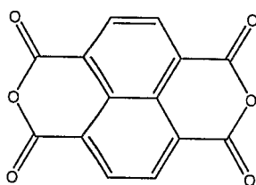
(1,4,5,8—naphthalene tetracarboxylic dianhydride)
