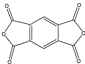
(pyromellitic dianhydride—PMDA)
