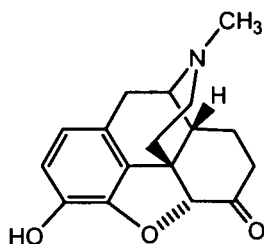
hydromorphone (7,8-dihydromorphin-6-one);
