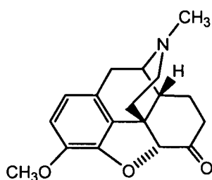
hydrocodone (3-methyl-7,8-dihydromorphin-6-one);
