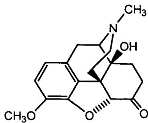
oxycodone (14-hydroxy-3-methyl-7,8-dihydromorphin-6-one).
