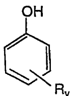
Formula I
