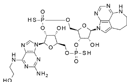
16 16a (Diastereomer 1) 16b (Diastereomer 2)
