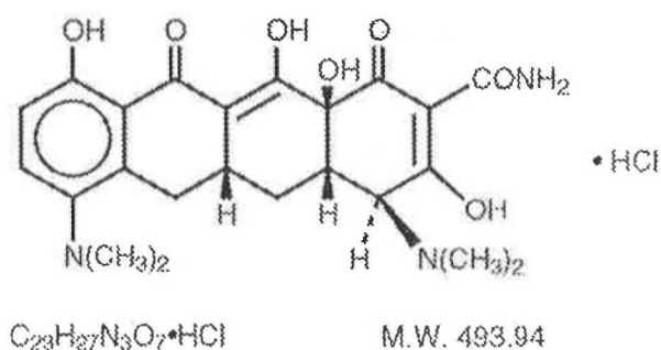
25 Structure of Minocycline HCl
