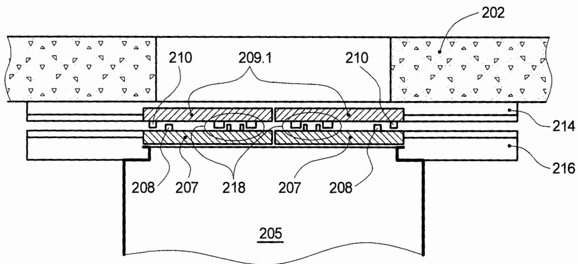
Fig. 3 (Section III-III)
