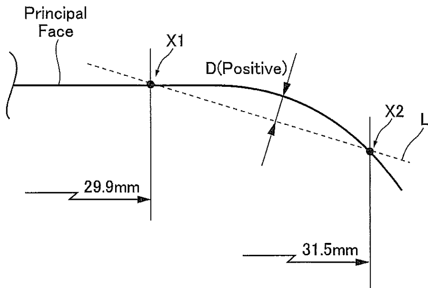
ROLL-OFF SHAPE
