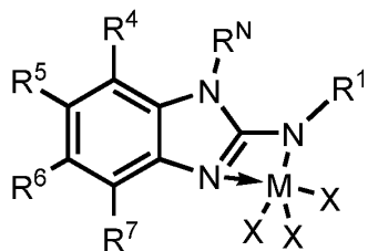
(IIc)
