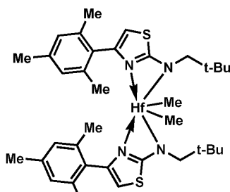
Procatalyst 20
