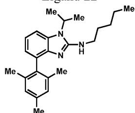
Ligand 25
