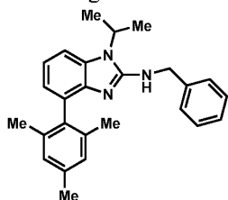
Ligand 31
