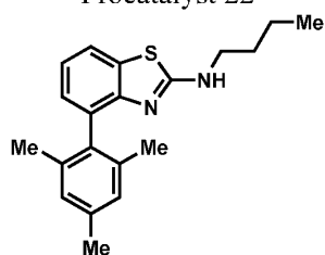
Ligand 1
