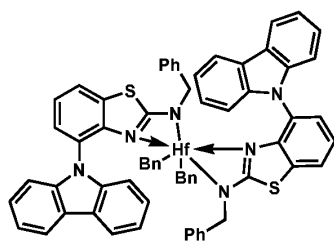
Procatalyst 19
