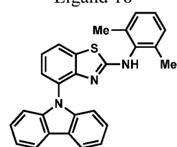
Ligand 21
