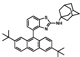
Ligand 22
