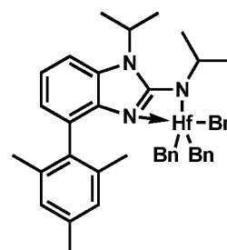
Procatalyst 21
