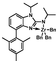
Procatalyst 22
