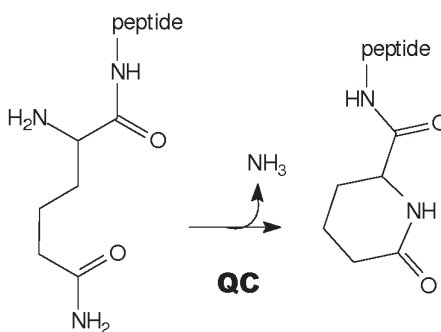
Scheme 2: Cyclization of L-homoglutamine by QC
