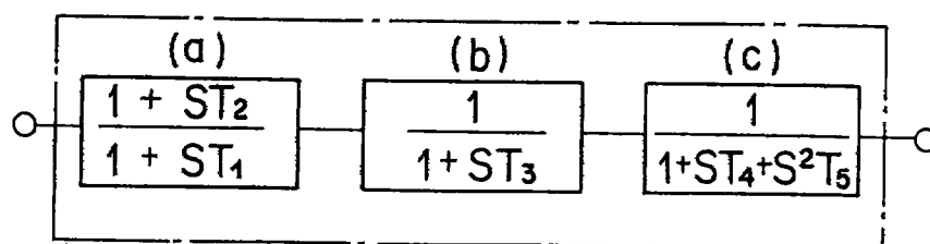
LOW-BAND COMPENSATION CIRCUIT
