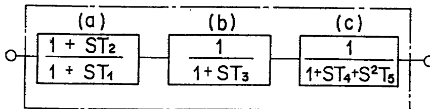
LOW-BAND COMPENSATION CIRCUIT
