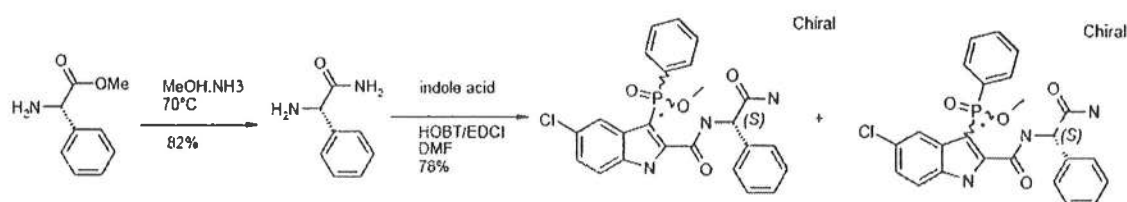
Scheme 26
