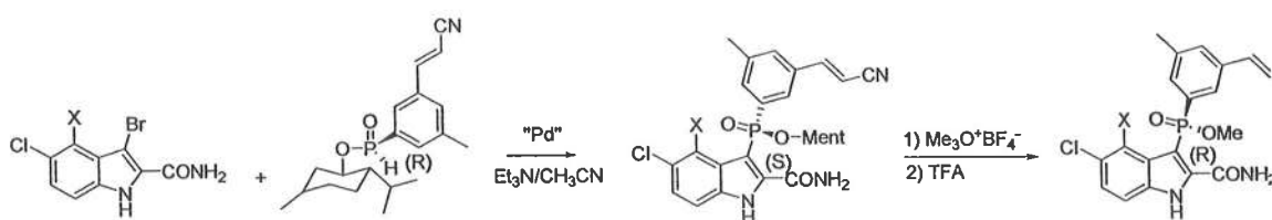
Scheme 24
