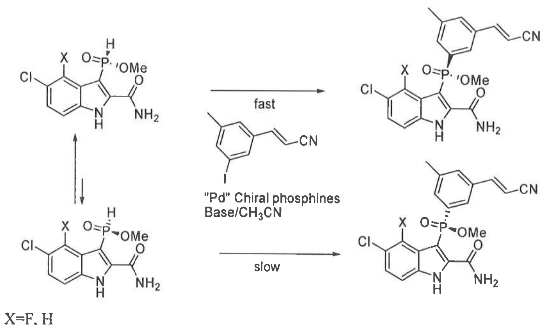
Scheme 12
