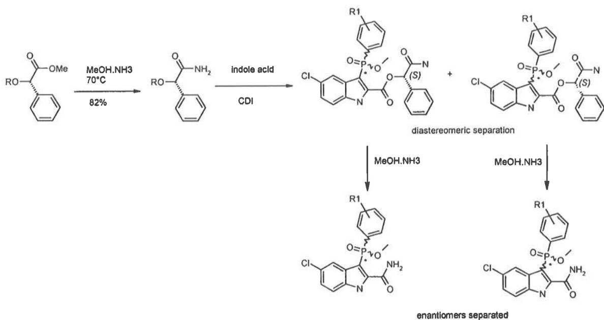
Scheme 27
