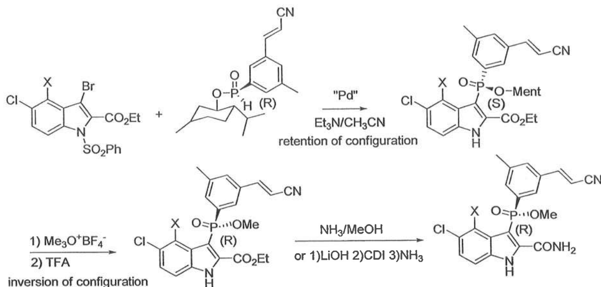
Scheme 25
