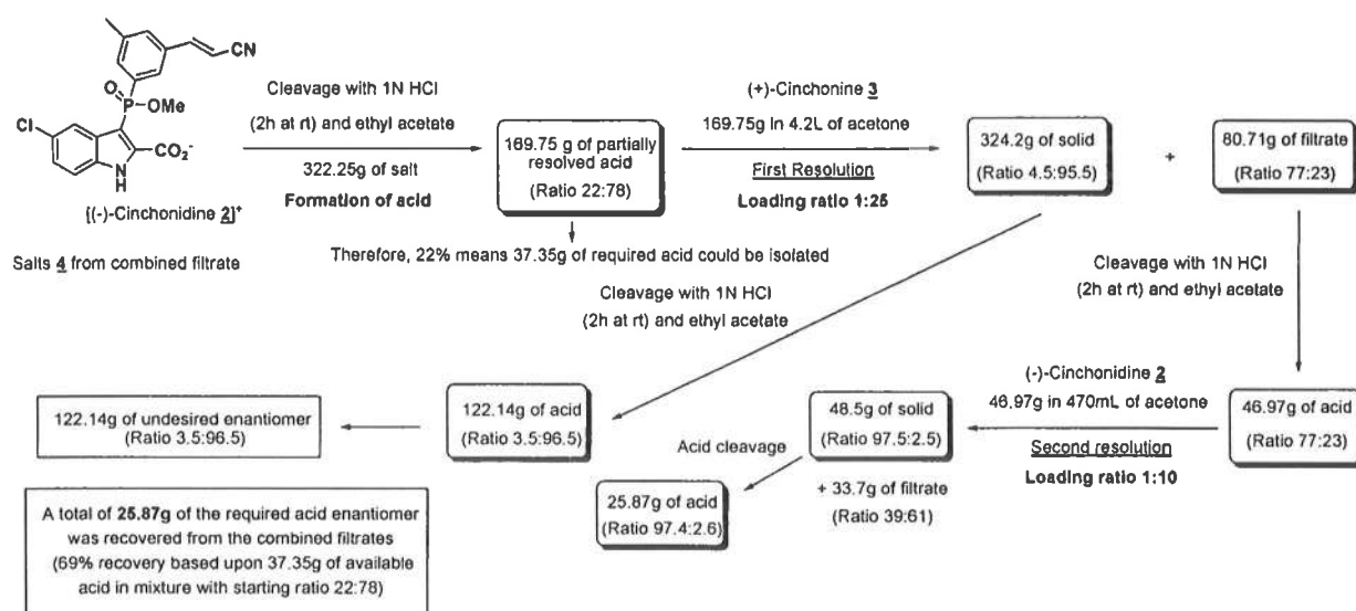
Scheme 16
