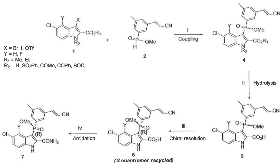
Scheme 3
