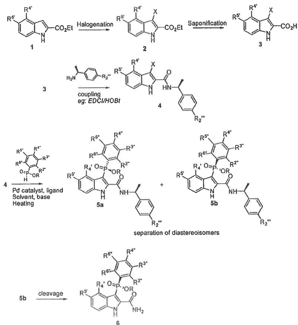
Scheme 13
