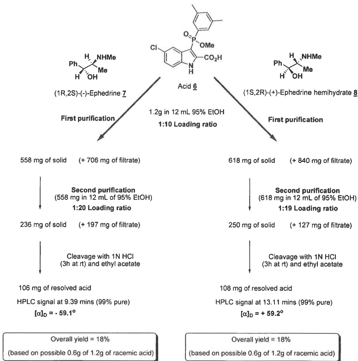
Scheme 19
