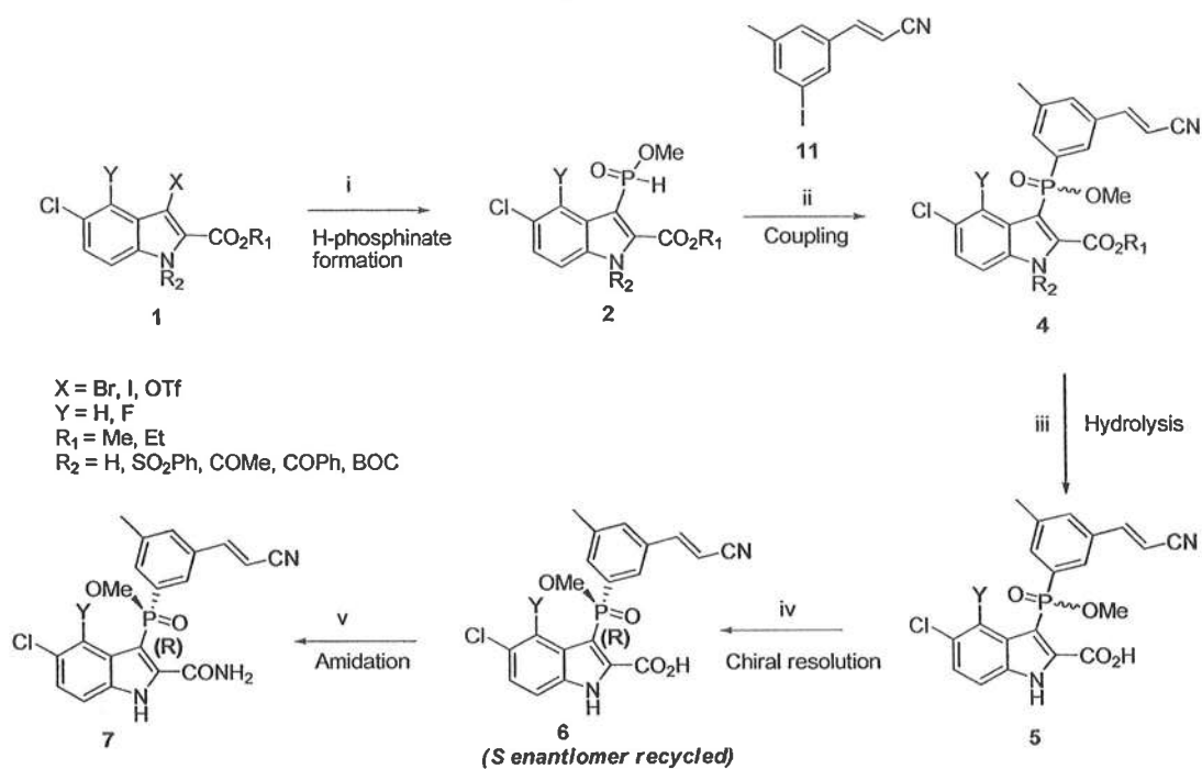
Scheme 2
