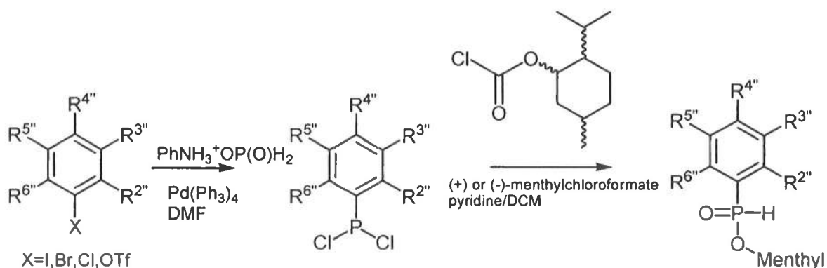
Scheme 21
