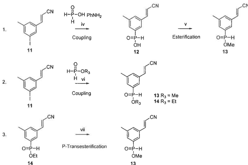
Scheme 4
