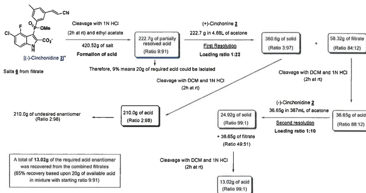
Scheme 18
