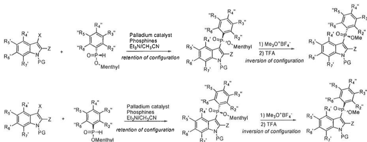
Scheme 20
