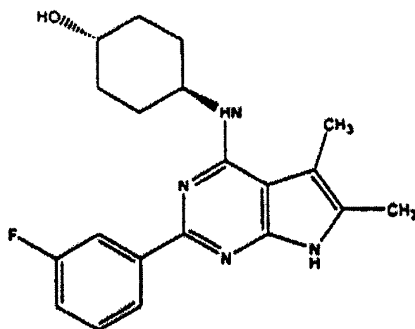
(Compound 706)
