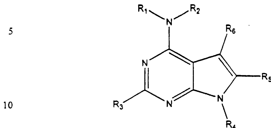
(I)
