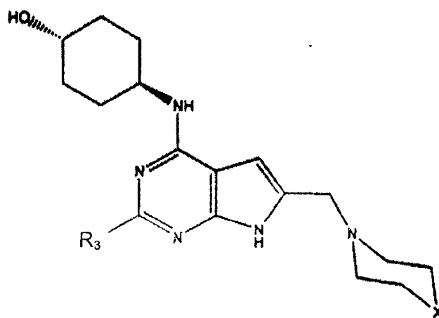
IX
