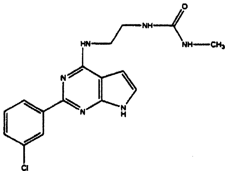
(Compound 1520)
