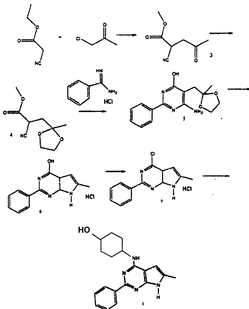
Scheme IV
