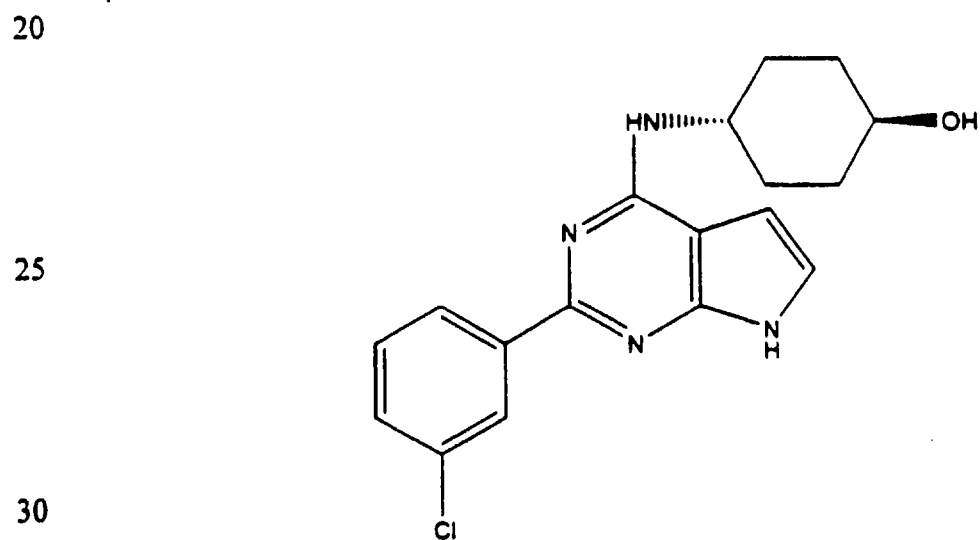
(Compound 1320)
