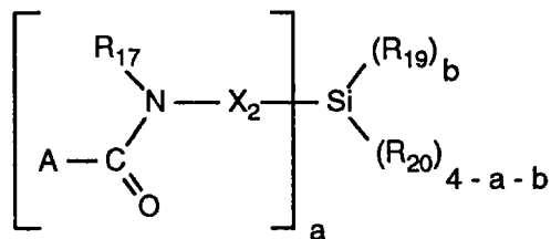
(VIb)
