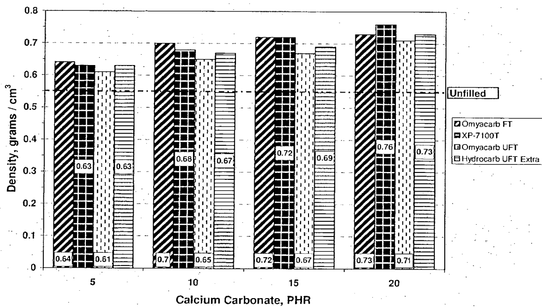
Effect of Calcium Carbonate on Density of Free Foam PVC 0.6 phr Azodicarbonmide
