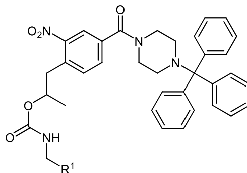
Formula (I)
