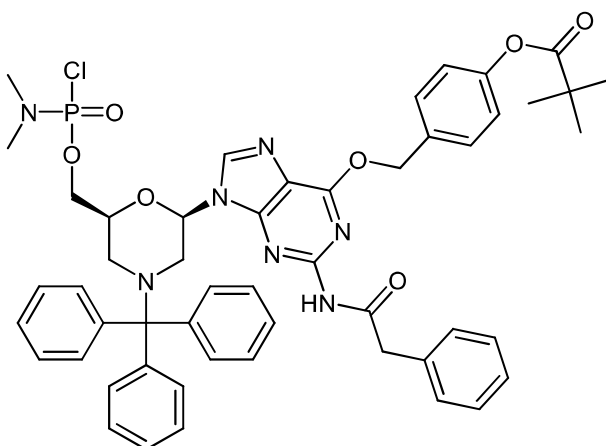
Compound (E1)
