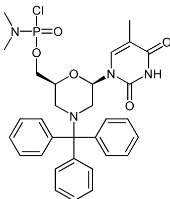
Compound (F1)
