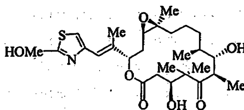
Epothilone F
