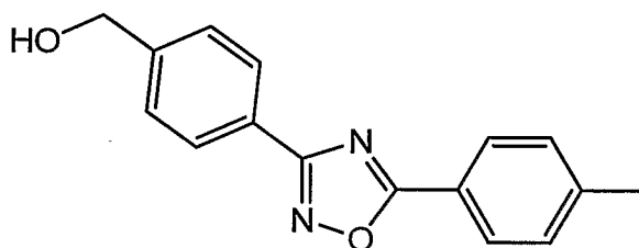
12A. {4-[5-(4-Methylphenyl)-1,2,4-oxadiazol-3-yl]phenyl}methanol
