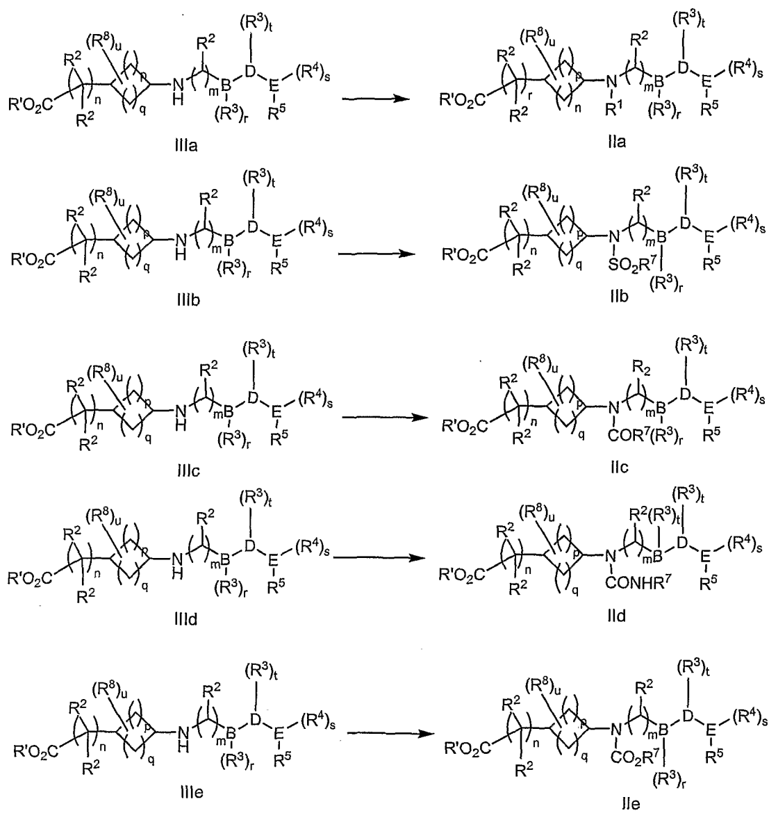
Scheme 12
