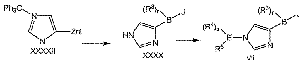
Scheme 11
