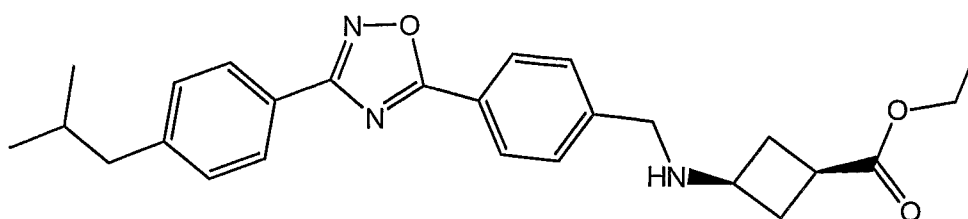
6A: Ethyl cis-3-((4-[3-(4-isobutylphenyl)-1,2,4-oxadiazol-5-yl]benzyl)amino)cyclobutanecarboxylate
