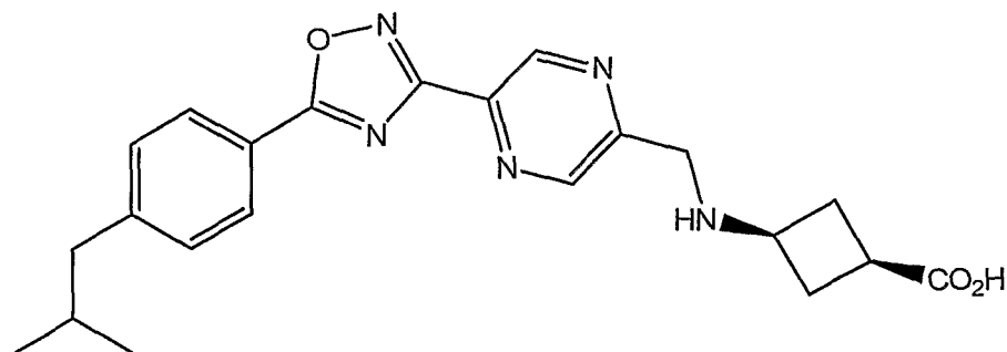
1B. 3-({5-[5-(4-isobutyl-phenyl)-[1,2,4]oxadiazol-3-yl]-pyrazin-2-ylmethyl}-amino)- cis -cyclobutanecarboxylic acid
