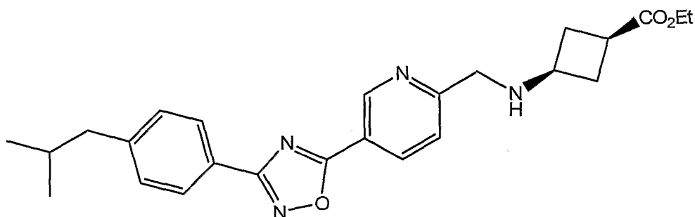
2A. 3-({5-[3-(4-isobutyl-phenyl)-[1,2,4]oxadiazole-5-yl]-pyridin-2-ylmethyl}-amino)- cis -cyclobutanecarboxylic acid ethyl ester
