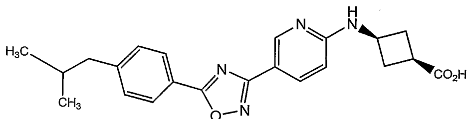
28A: 3-{5-[5-(4-Isobutyl-phenyl)-[1,2,4]oxadiazol-3-yl]-pyridin-2-ylamino}-cyclobutanecarboxylic acid hydrochloride
