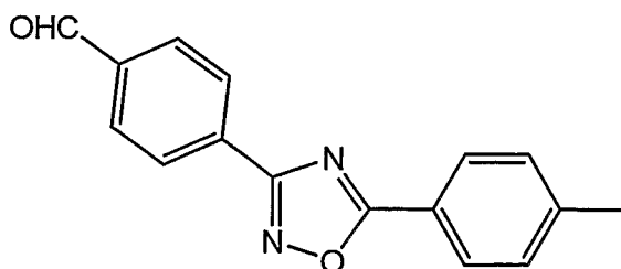
12B. 4-[5-(4-Methylphenyl)-1,2,4-oxadiazol-3-yl]benzaldehyde
