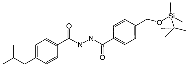
9C: 4-(tert-Butyl-dimethyl-silanyloxymethyl)-benzoic acid N'-(4-isobutyl-benzoyl)-hydrazide
