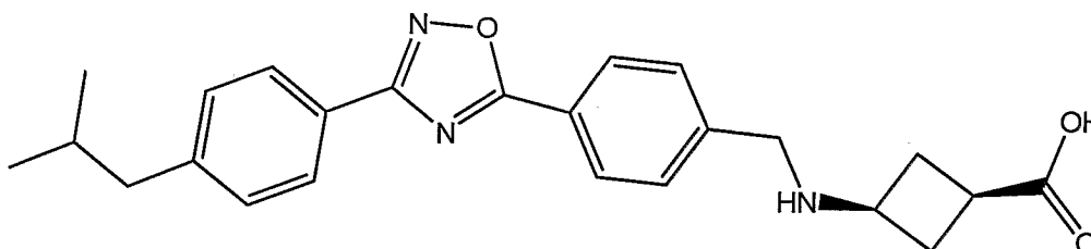
6B: cis-3-((4-[3-(4-Isobutylphenyl)-1,2,4-oxadiazol-5-yl]benzyl)amino)cyclobutanecarboxylic acid hydrochloride
