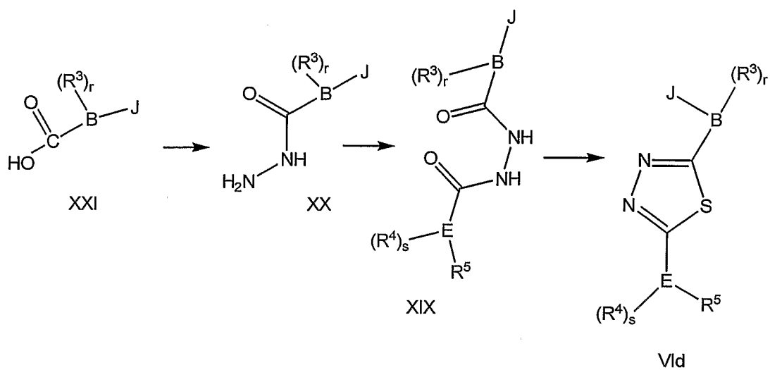
Scheme 6
