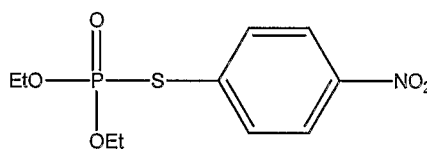
O,O'-diethyl-S-p-nitrophenylphosphothioate
