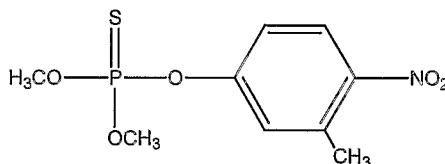
Fenitrothion
