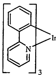
Chemical formula 3
