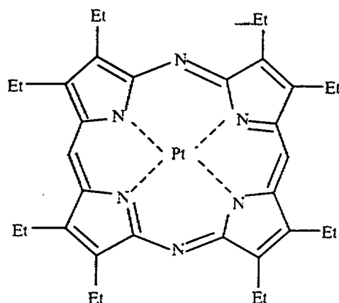
Chemical formula 2
