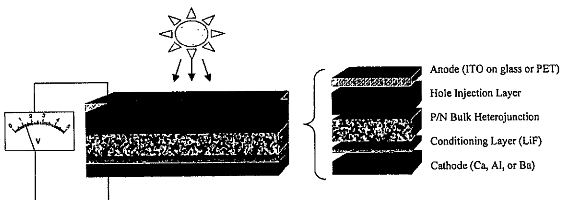
Figure 1: A typical conductive polymer photovoltaic (solar) cell
