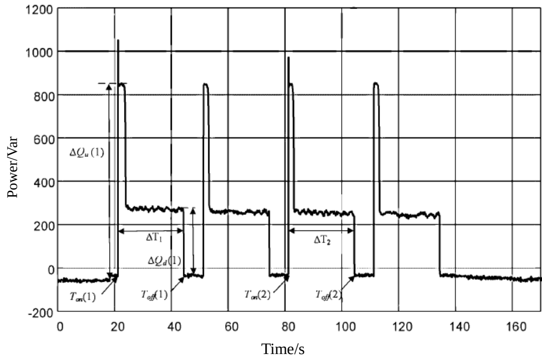
Reactive Power of Microwave Oven
