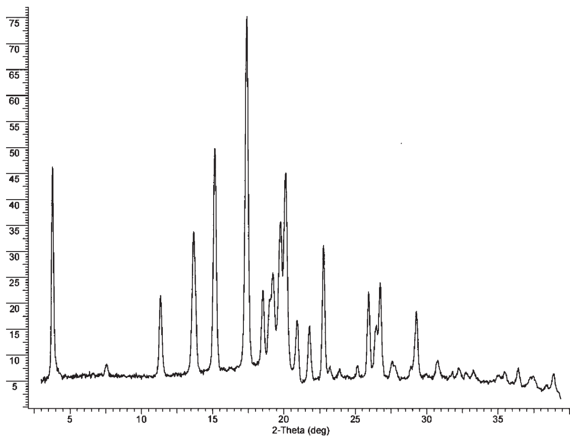
Figure 1: Fumarate
