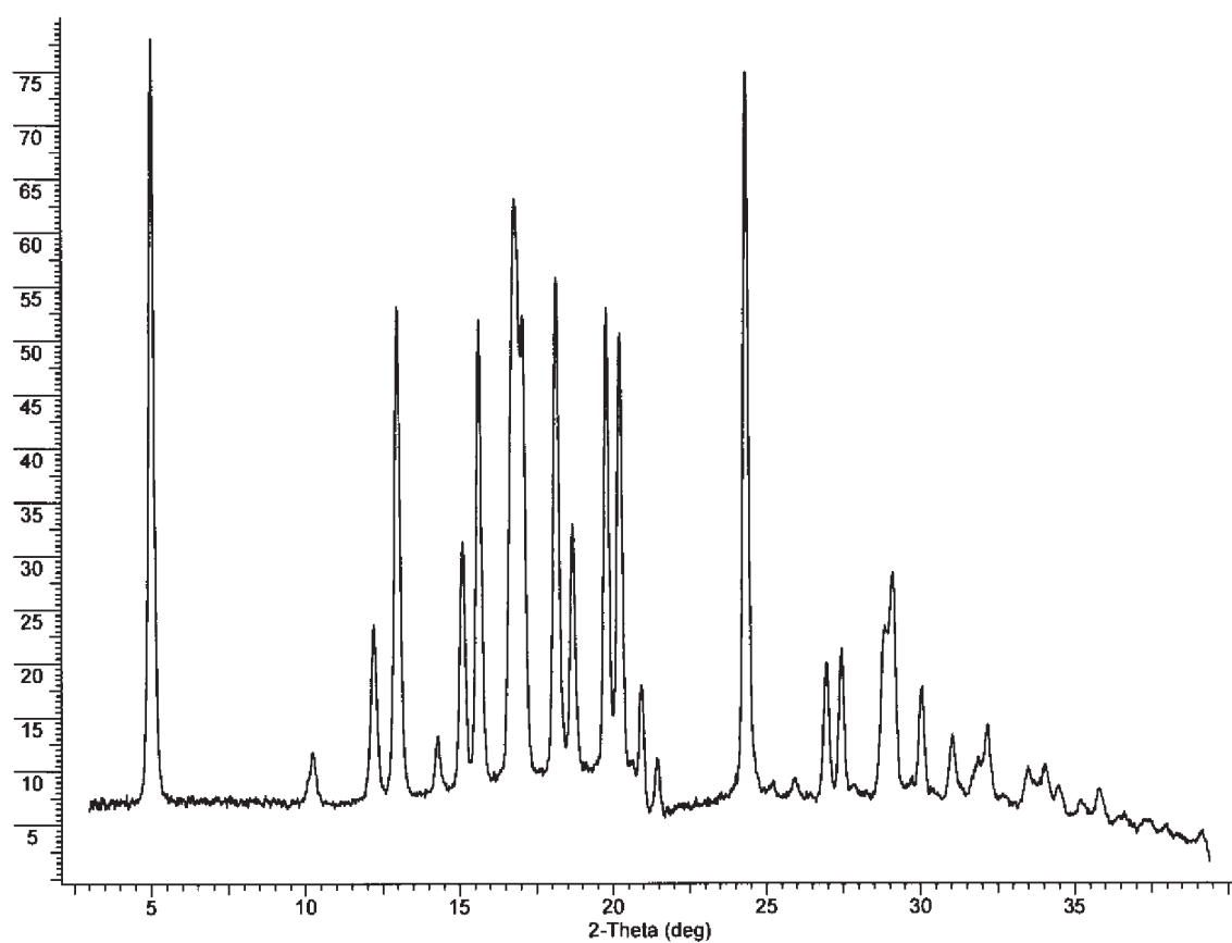
Figure 6: Malonate
