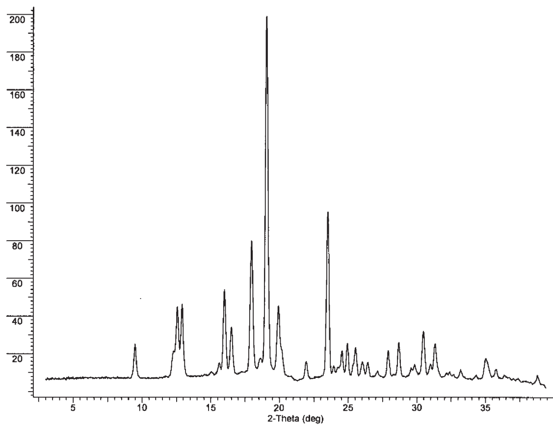
Figure 2: Maleate
