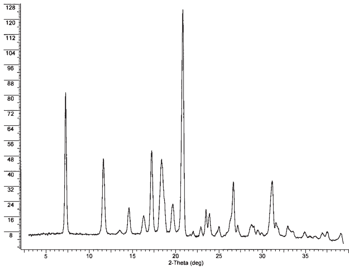
Figure 3: Hydrochloride
