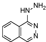
Hydralazine.
