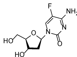
5-fluoro-2'-deoxycytidine
