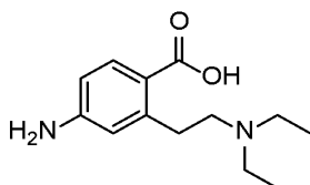
Procaine.
