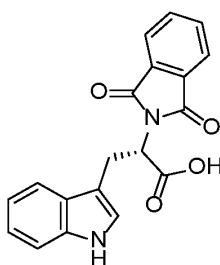
RG108.
