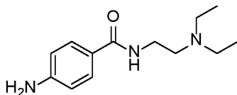
Procainamide.
