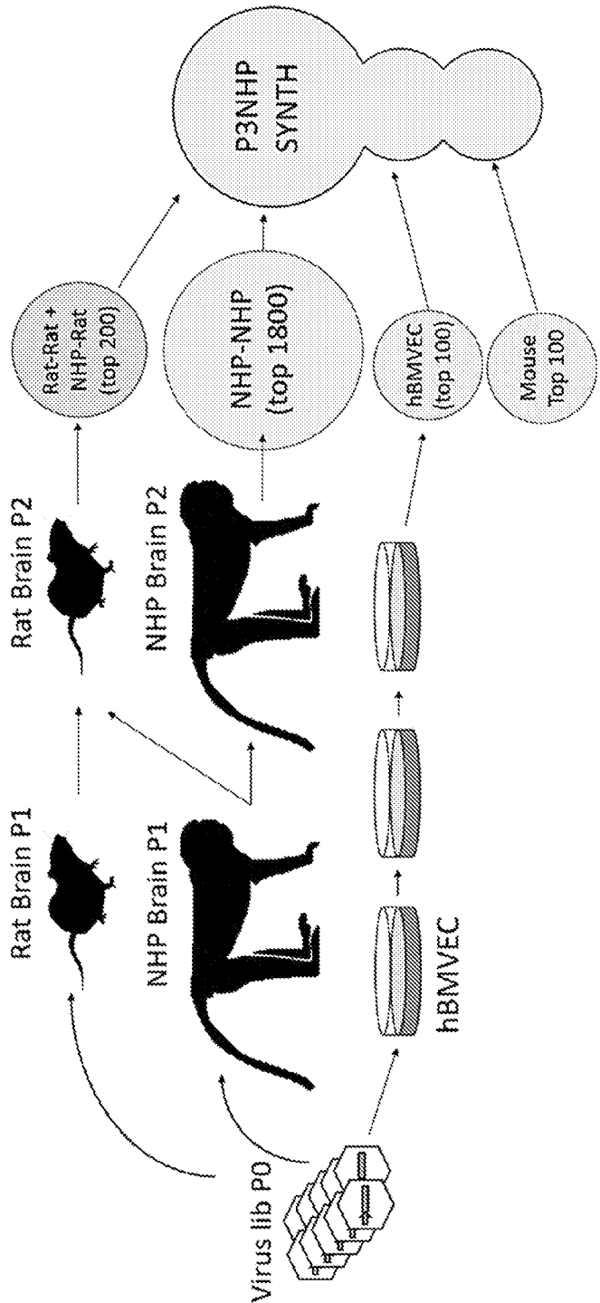
FIG. 2 Orthogonal Evolution of Loop8-7mer Library
