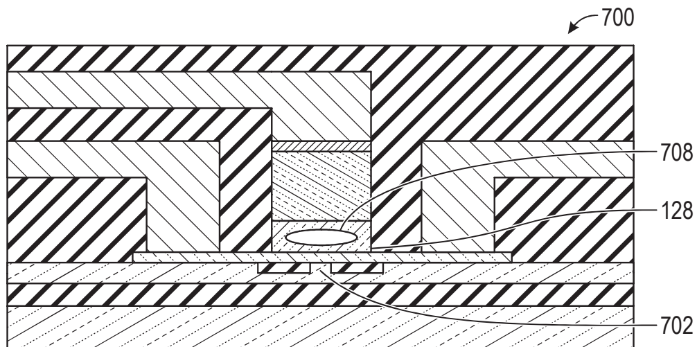
SECTION C-C FIG. 7C
