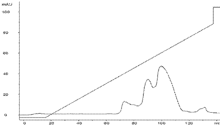
Figure 5: CEX chromatogram of separation on SP Sepharose HP
