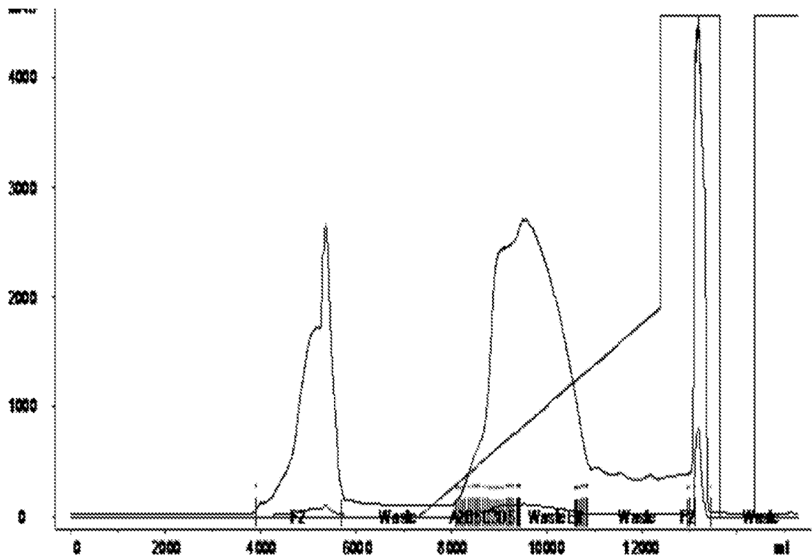
Figure 4: Preparative CEX chromatogram of separation on Toyopearl SP65S
