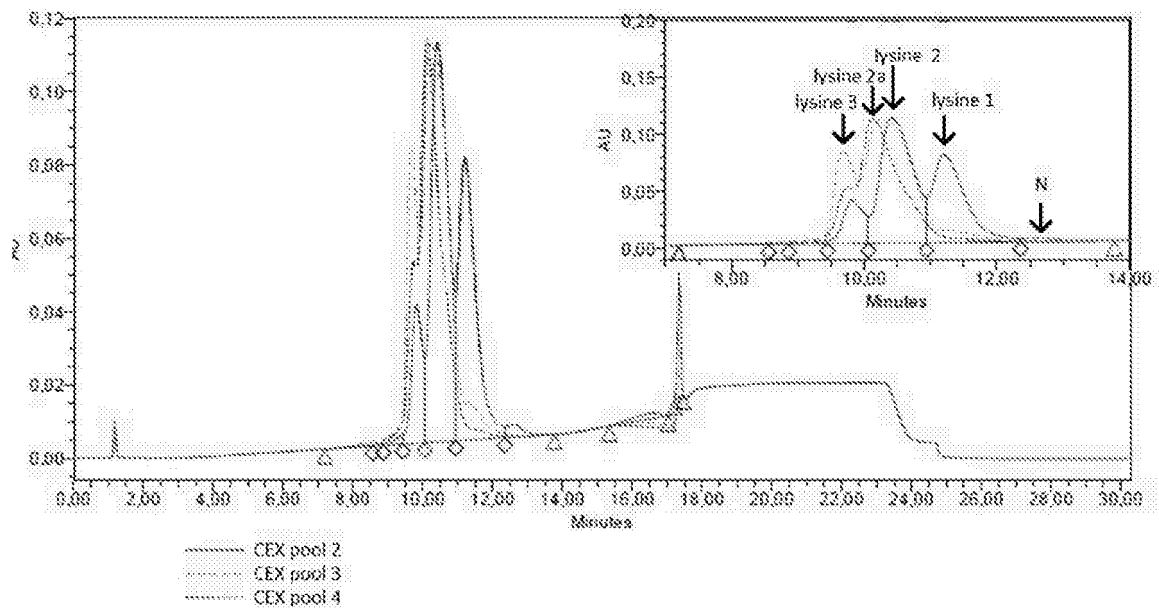
Figure 3: CE-HPLC analysis of pooled material from preparative CEX isolation of monoPEG-IGF1 isoforms.
