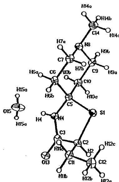
Structure 1: ORTEP structure of C_{10}H_{18}N_2OS + H_2O
