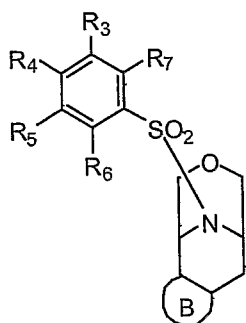
Formula VIIIe
