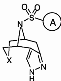
Formula VIIa
