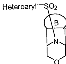
Formula Ve
