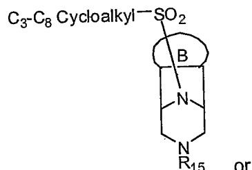
Formula IVd
