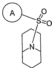
Formula VII
