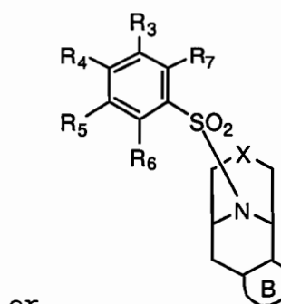
Formula VIIIb
