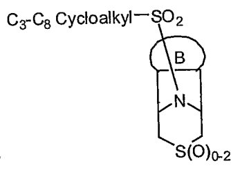
Formula IVf
