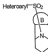
Formula Vc
