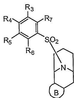
Formula VIIIc
