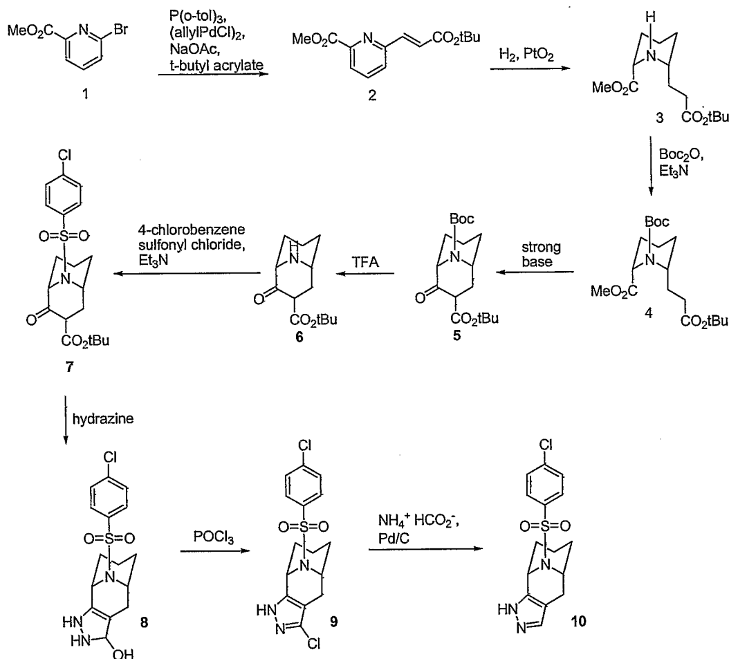
Scheme 2
