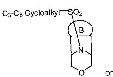
Formula IVe
