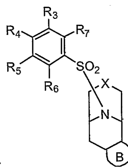
Formula VIIIb
