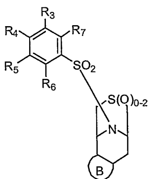
Formula VIIIg
