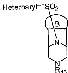
Formula Vd
