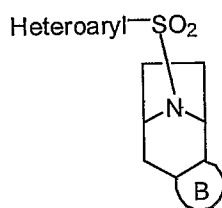
Formula Vb
