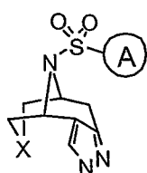
Formula VIIa
