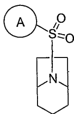
Formula II,
