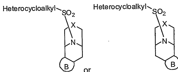
Formula XIb
