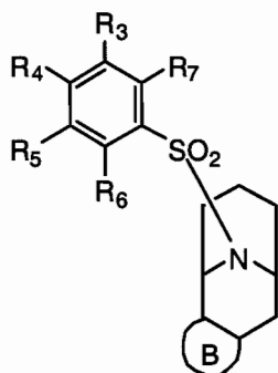
Formula VIIIc
