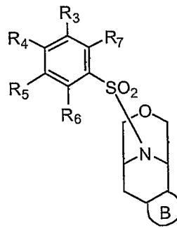
Formula VIIIf,
