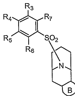
Formula VIIIId,
