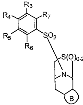
Formula VIIIh
