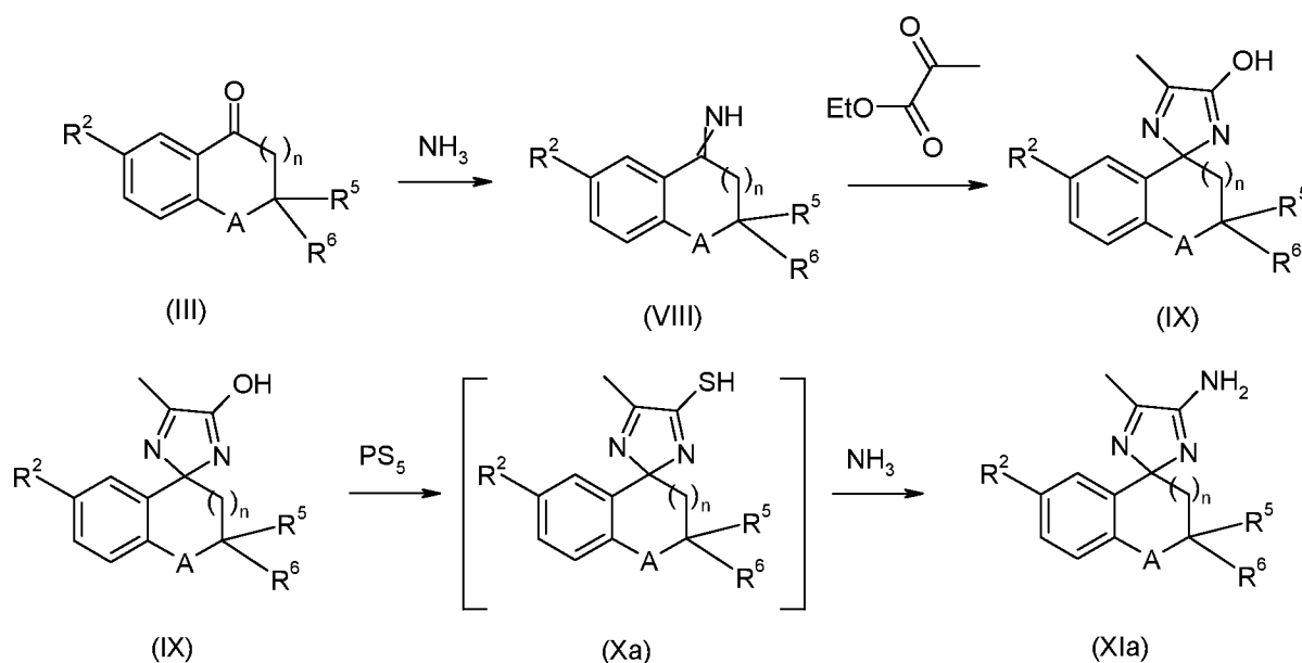
Scheme 4
