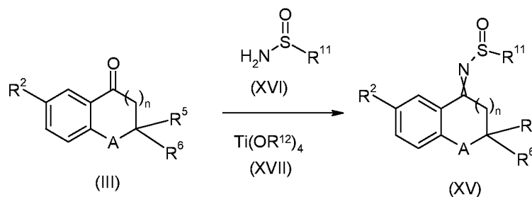
Scheme 7
