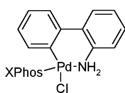
precatalyst 13
