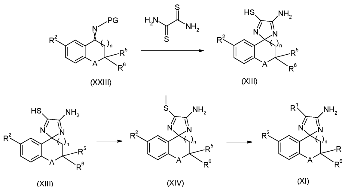
Scheme 13
