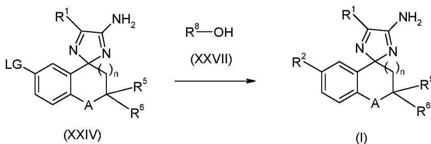
Scheme 17
