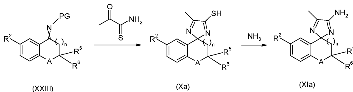
Scheme 12
