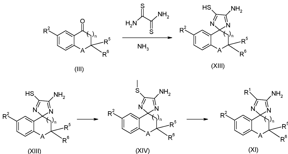
Scheme 5
