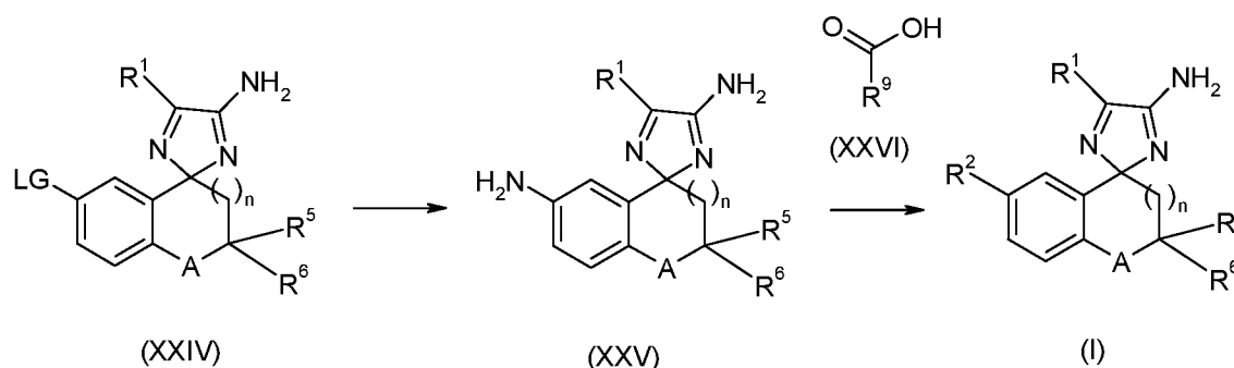
Scheme 15
