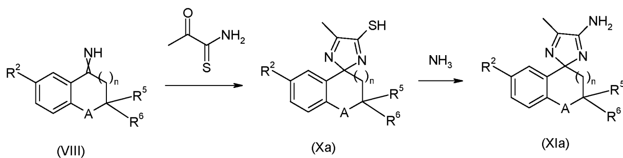
Scheme 11
