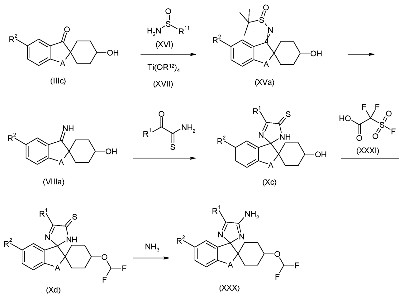
Scheme 20
