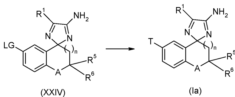
Scheme 14a
