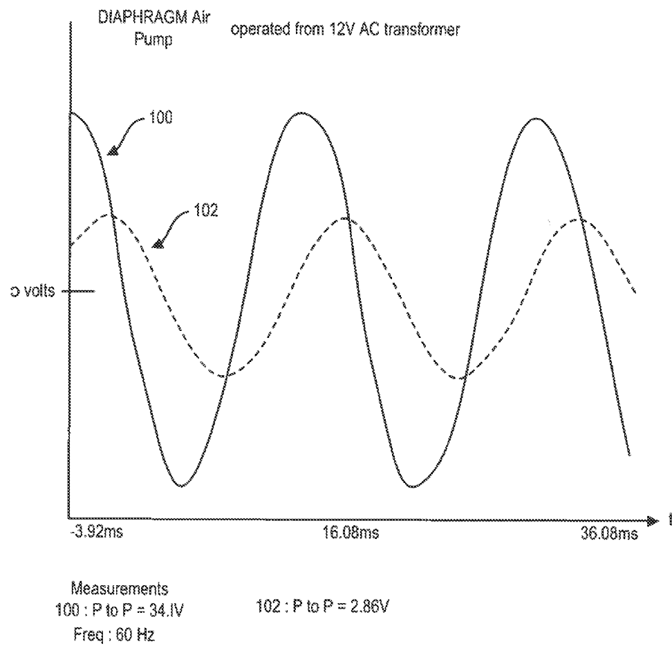
PRIOR ART FIG. 2
