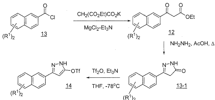
Scheme 5
