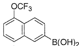
Intermediate C
