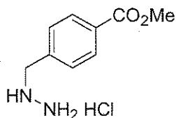
Intermediate N
