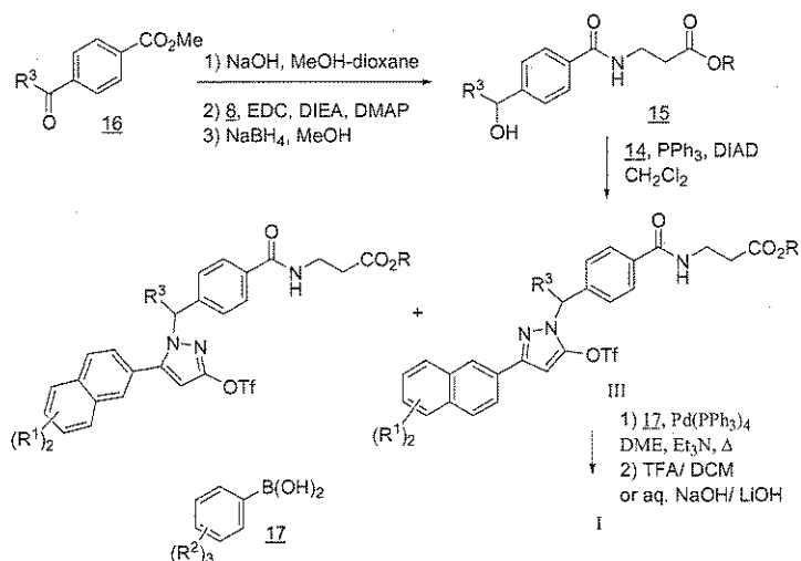
Scheme 6
