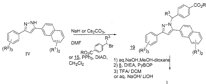
Scheme 11
