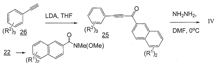
Scheme 10
