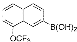
Intermediate D
