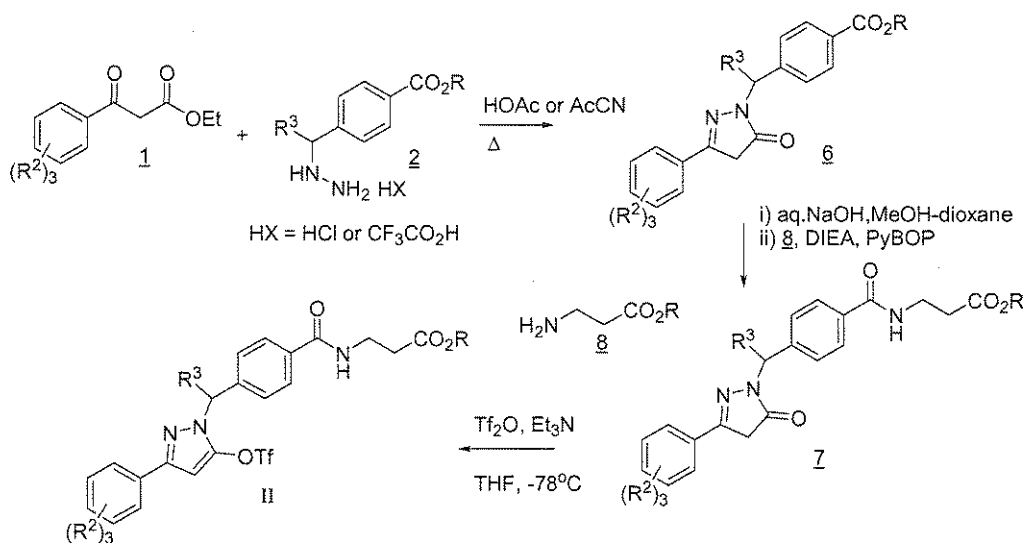
Scheme 3
