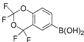
Intermediate E
