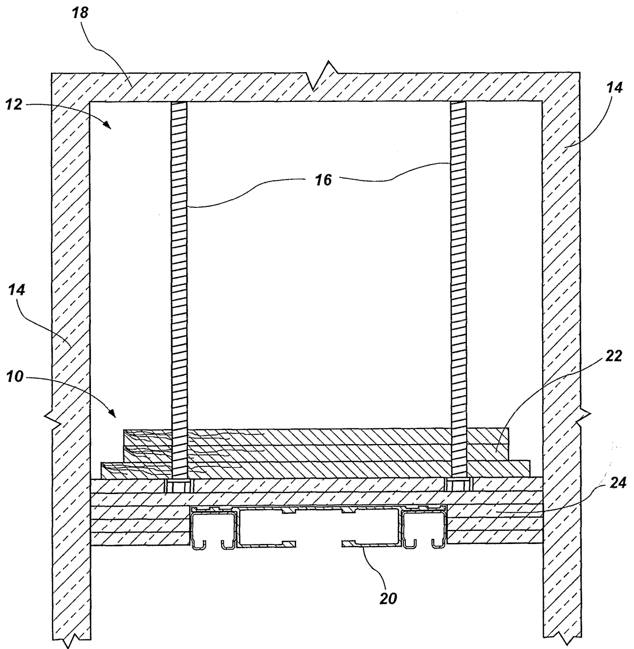
FIG. 1 (PRIOR ART)
