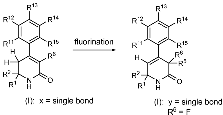
Scheme 10
