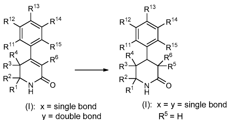
Scheme 11
