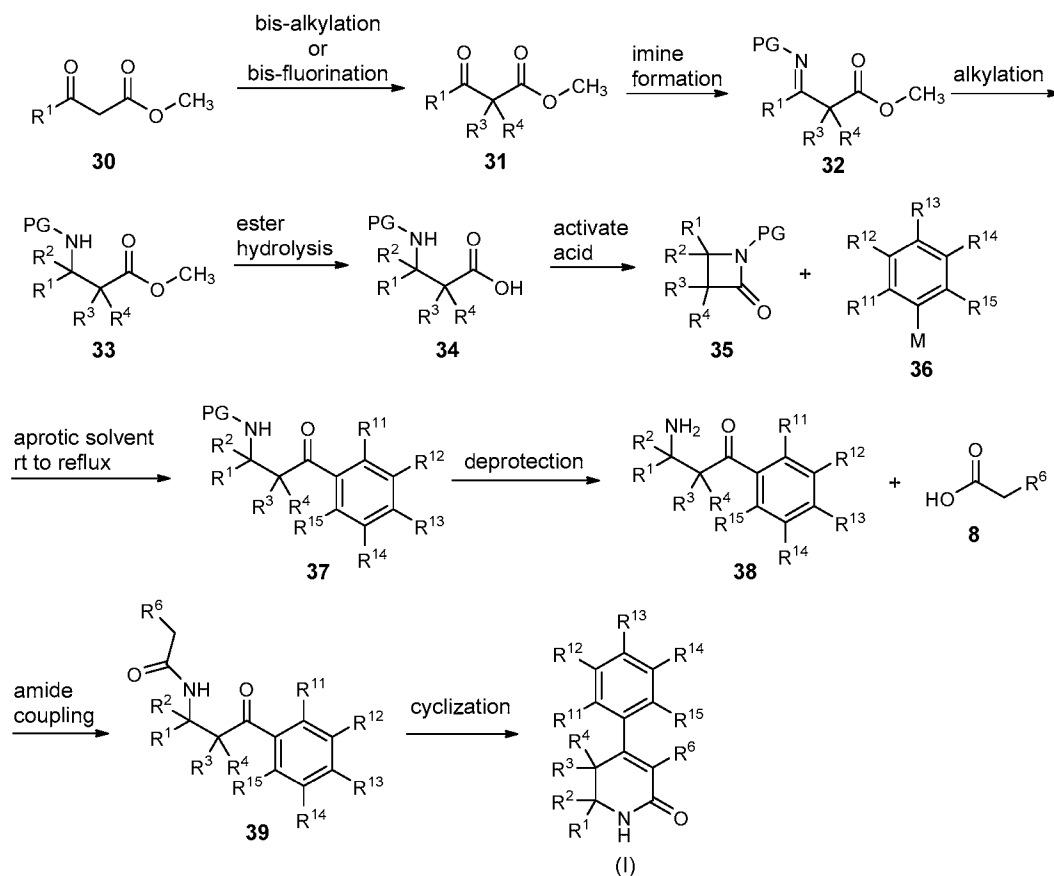
Scheme 9
