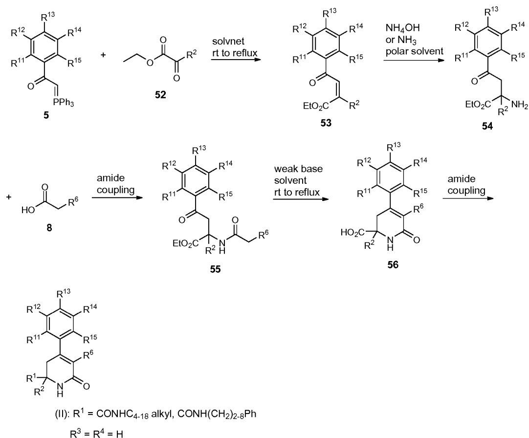
Scheme 14
