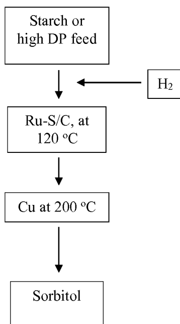
Figure 1: Scheme for Synthesis of Sorbitol from Starch or Maltodextrin Feed Using Ru-S/C and Copper Catalyst
