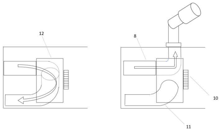
Fig 5: Side profile showing rotary valve in different modes
