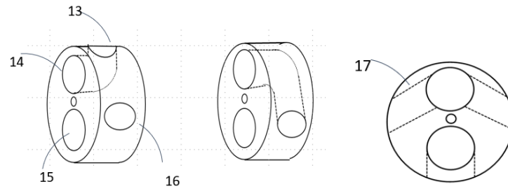
Fig 4 : Rotary Valve
