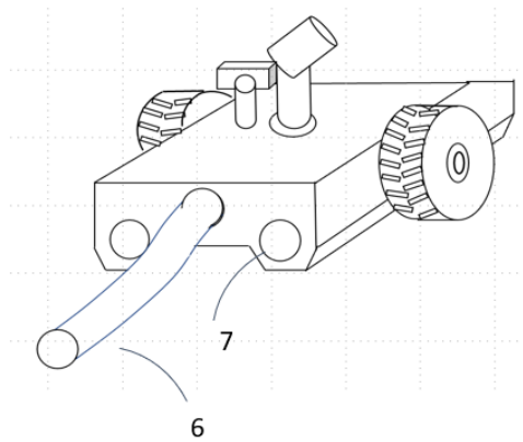
Figure 2 : Rear Perspective of Marine Fire Fighting Robot
