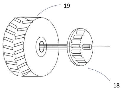
Fig 6 : Robot wheel attached to paddle wheel drive
