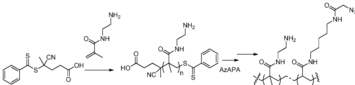
Scheme 2.1.
