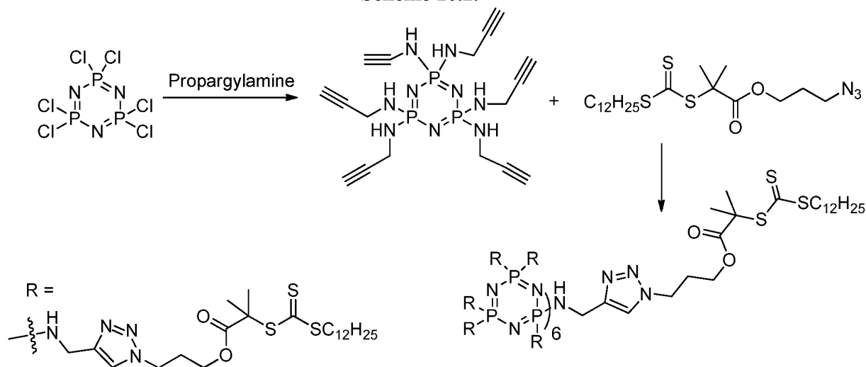
Scheme 10.2.
