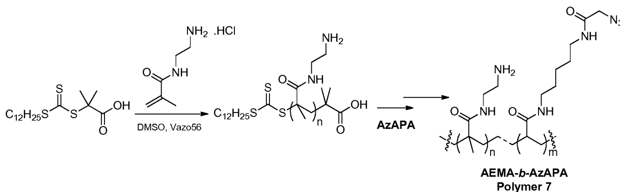
Scheme 2.2.
