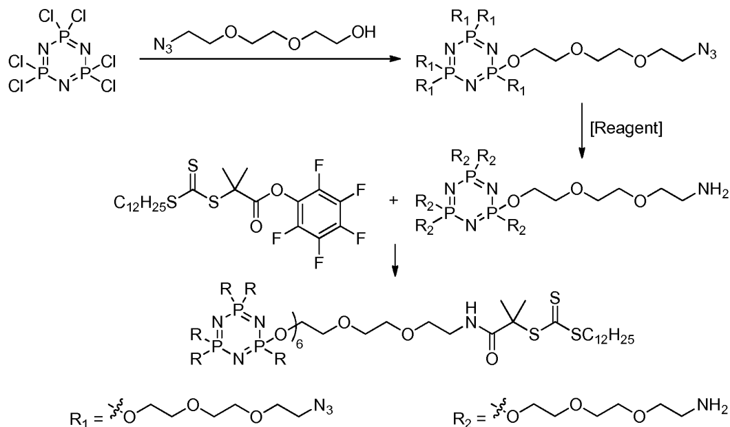
Scheme 10.3.
