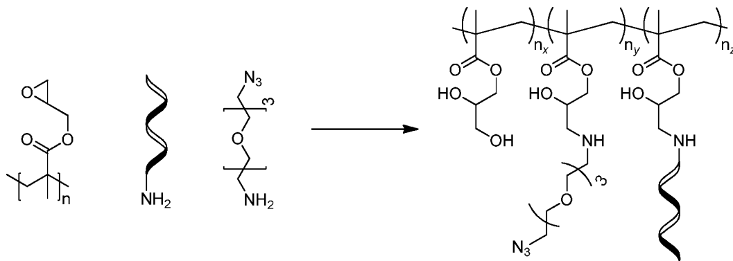
Scheme 8. Preparation of Pre-grafted Poly(Glycidyl Methacrylate)
