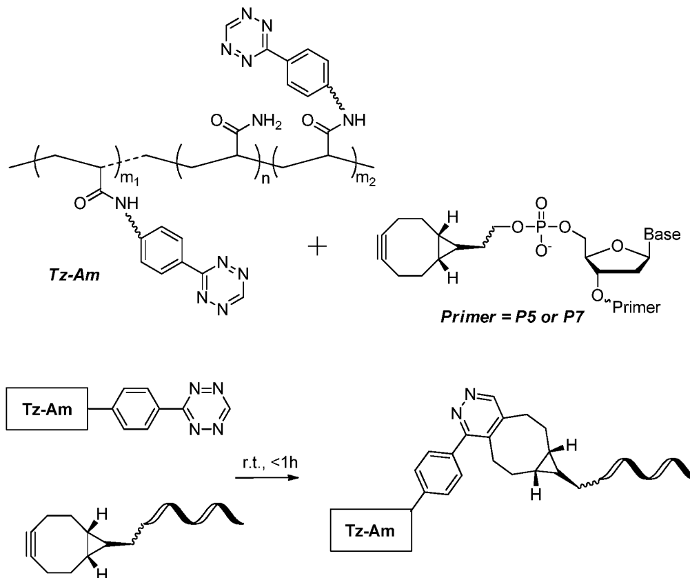
Scheme 4. Oligo Reaction with Tetrazine-Functionalized Polymer
